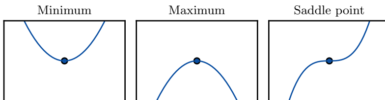
Figure 4.2: Types of critical points. Examples of the three types of critical points in one dimension. A critical point is a point with zero slope. Such a point can either be a local minimum, which is lower than the neighboring points; a local maximum, which is higher than the neighboring points; or a saddle point, which has neighbors that are both higher and lower than the point itself.
