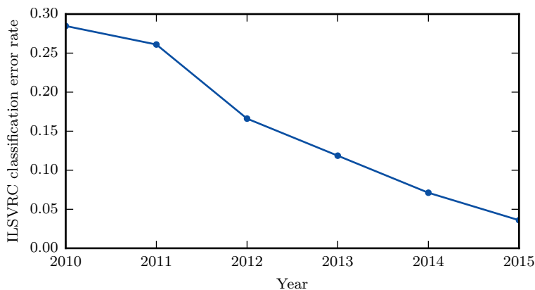
Figure 1.12: Decreasing error rate over time. Since deep networks reached the scale necessary to compete in the ImageNet Large Scale Visual Recognition Challenge, they have consistently won the competition every year, yielding lower and lower error rates each time. Data from Russakovsky et al. (2014b) and He et al. (2015).
