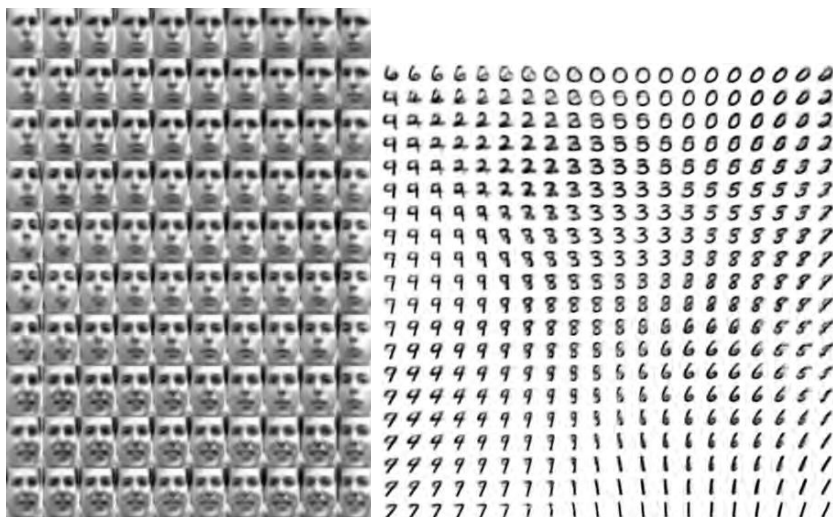
Figure 20.6: Examples of 2-D coordinate systems for high-dimensional manifolds, learned by a variational autoencoder (Kingma and Welling, 2014a). Two dimensions may be plotted directly on the page for visualization, so we can gain an understanding of how the model works by training a model with a 2-D latent code, even if we believe the intrinsic dimensionality of the data manifold is much higher. The images shown are not examples from the training set but images \mathbf{x} actually generated by the model p(\mathbf{x} | \mathbf{z}) , simply by changing the 2-D “code” \mathbf{z} (each image corresponds to a different choice of “code” \mathbf{z} on a 2-D uniform grid). (Left) The 2-D map of the Frey faces manifold. One dimension that has been discovered (horizontal) mostly corresponds to a rotation of the face, while the other (vertical) corresponds to the emotional expression. (Right) The 2-D map of the MNIST manifold.
