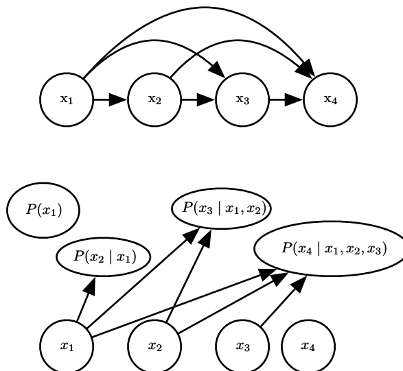
Figure 20.8: A fully visible belief network predicts the i -th variable from the i - 1 previous ones. ( Top )The directed graphical model for an FVBN. ( Bottom )Corresponding computational graph for the logistic FVBN, where each prediction is made by a linear predictor.
