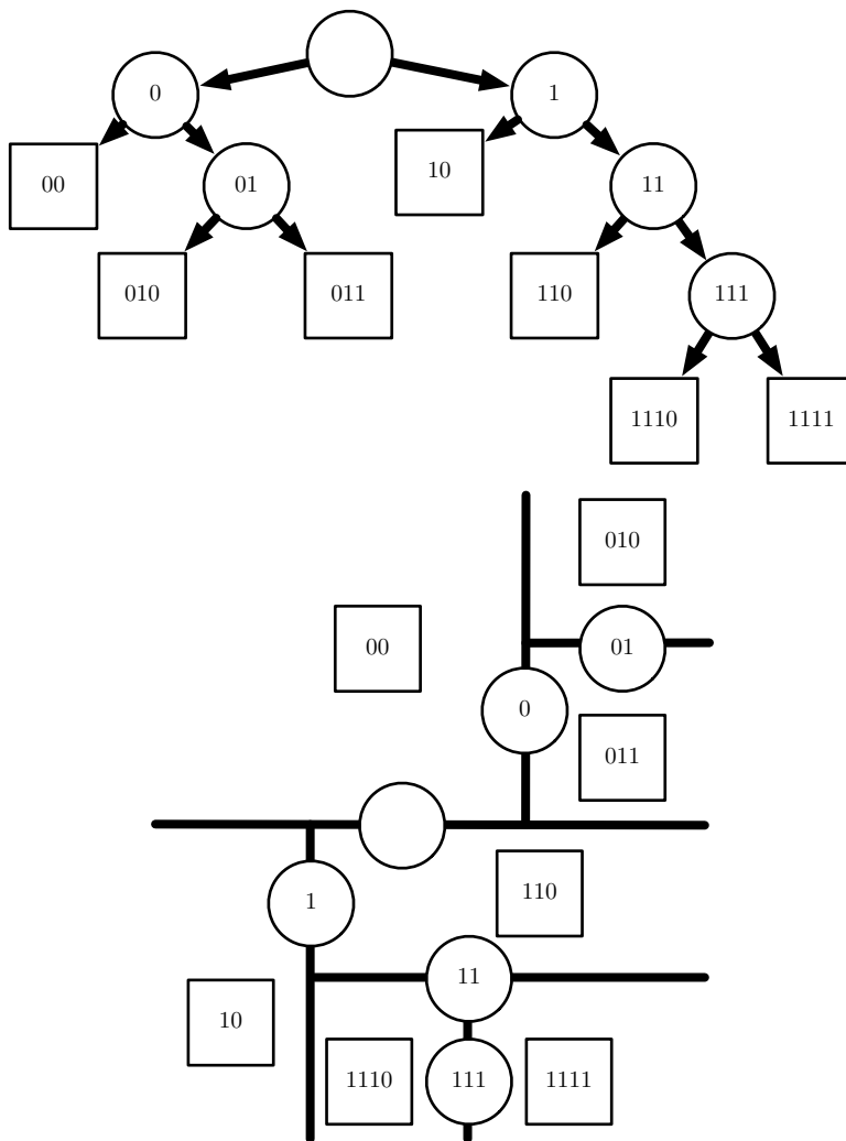
Figure 5.7: Diagrams describing how a decision tree works. ( Top )Each node of the tree chooses to send the input example to the child node on the left (0) or to the child node on the right (1). Internal nodes are drawn as circles and leaf nodes as squares. Each node is displayed with a binary string identifier corresponding to its position in the tree, obtained by appending a bit to its parent identifier (0 = choose left or top, 1 = choose right or bottom). ( Bottom )The tree divides space into regions. The 2-D plane shows how a decision tree might divide \mathbb{R}^2 . The nodes of the tree are plotted in this plane, with each internal node drawn along the dividing line it uses to categorize examples, and leaf nodes drawn in the center of the region of examples they receive. The result is a piecewise-constant function, with one piece per leaf. Each leaf requires at least one training example to define, so it is not possible for the decision tree to learn a function that has more local maxima than the number of training examples.
