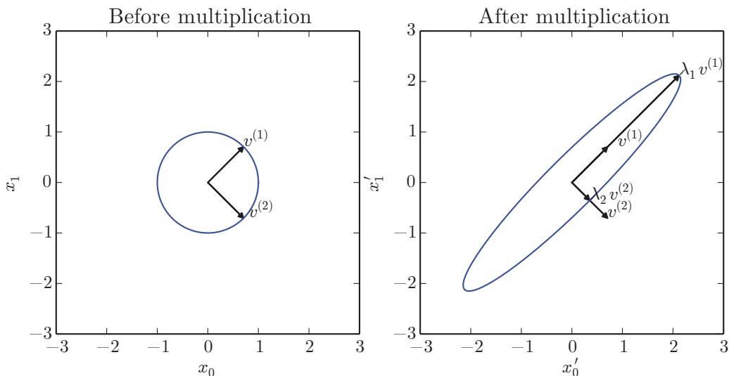
Figure 2.3: Effect of eigenvectors and eigenvalues. An example of the effect of eigenvectors and eigenvalues. Here, we have a matrix \mathbf{A} with two orthonormal eigenvectors, \mathbf{v}^{(1)} with eigenvalue \lambda_1 and \mathbf{v}^{(2)} with eigenvalue \lambda_2 . ( Left ) We plot the set of all unit vectors \mathbf{u} \in \mathbb{R}^2 as a unit circle. ( Right ) We plot the set of all points \mathbf{A}\mathbf{u} . By observing the way that \mathbf{A} distorts the unit circle, we can see that it scales space in direction \mathbf{v}^{(i)} by \lambda_i .
