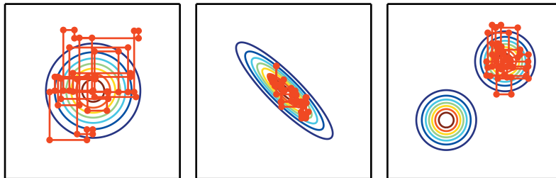
Figure 17.1: Paths followed by Gibbs sampling for three distributions, with the Markov chain initialized at the mode in both cases. (Left) A multivariate normal distribution with two independent variables. Gibbs sampling mixes well because the variables are independent. (Center) A multivariate normal distribution with highly correlated variables. The correlation between variables makes it difficult for the Markov chain to mix. Because the update for each variable must be conditioned on the other variable, the correlation reduces the rate at which the Markov chain can move away from the starting point. (Right) A mixture of Gaussians with widely separated modes that are not axis aligned. Gibbs sampling mixes very slowly because it is difficult to change modes while altering only one variable at a time.
