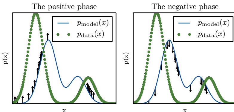
Figure 18.1: The view of algorithm 18.1 as having a “positive phase” and a “negative phase.” ( Left ) In the positive phase, we sample points from the data distribution and push up on their unnormalized probability. This means points that are likely in the data get pushed up on more. ( Right ) In the negative phase, we sample points from the model distribution and push down on their unnormalized probability. This counteracts the positive phase’s tendency to just add a large constant to the unnormalized probability everywhere. When the data distribution and the model distribution are equal, the positive phase has the same chance to push up at a point as the negative phase has to push down. When this occurs, there is no longer any gradient (in expectation), and training must terminate.
