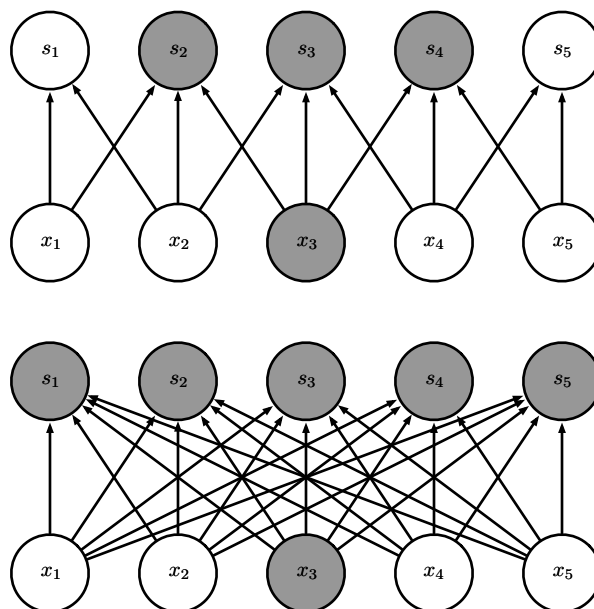
Figure 9.2: Sparse connectivity, viewed from below. We highlight one input unit, x_3 , and highlight the output units in s that are affected by this unit. ( Top )When s is formed by convolution with a kernel of width 3, only three outputs are affected by x . ( Bottom )When s is formed by matrix multiplication, connectivity is no longer sparse, so all the outputs are affected by x_3 .
