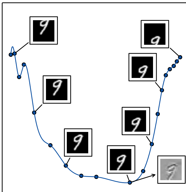
Figure 14.6: An illustration of the concept of a tangent hyperplane. Here we create a 1-D manifold in 784-D space. We take an MNIST image with 784 pixels and transform it by translating it vertically. The amount of vertical translation defines a coordinate along a 1-D manifold that traces out a curved path through image space. This plot shows a few points along this manifold. For visualization, we have projected the manifold into 2-D space using PCA. An n -dimensional manifold has an n -dimensional tangent plane at every point. This tangent plane touches the manifold exactly at that point and is oriented parallel to the surface at that point. It defines the space of directions in which it is possible to move while remaining on the manifold. This 1-D manifold has a single tangent line. We indicate an example tangent line at one point, with an image showing how this tangent direction appears in image space. Gray pixels indicate pixels that do not change as we move along the tangent line, white pixels indicate pixels that brighten, and black pixels indicate pixels that darken.
