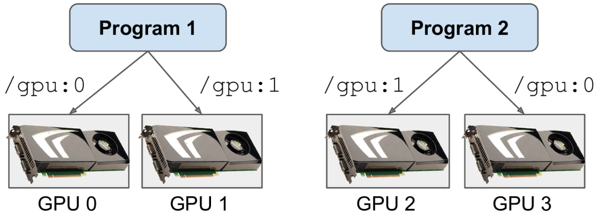
Figure 19-12. Each program gets two GPUs
