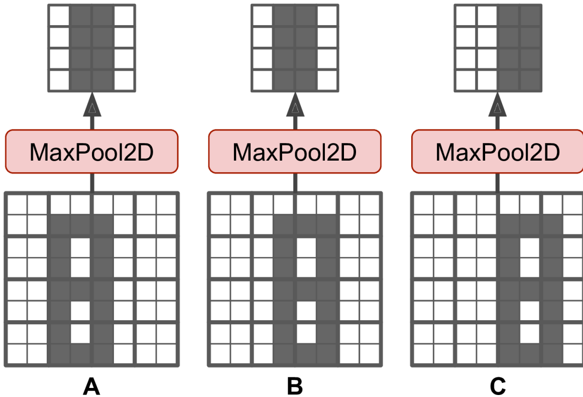
Figure 14-9. Invariance to small translations
