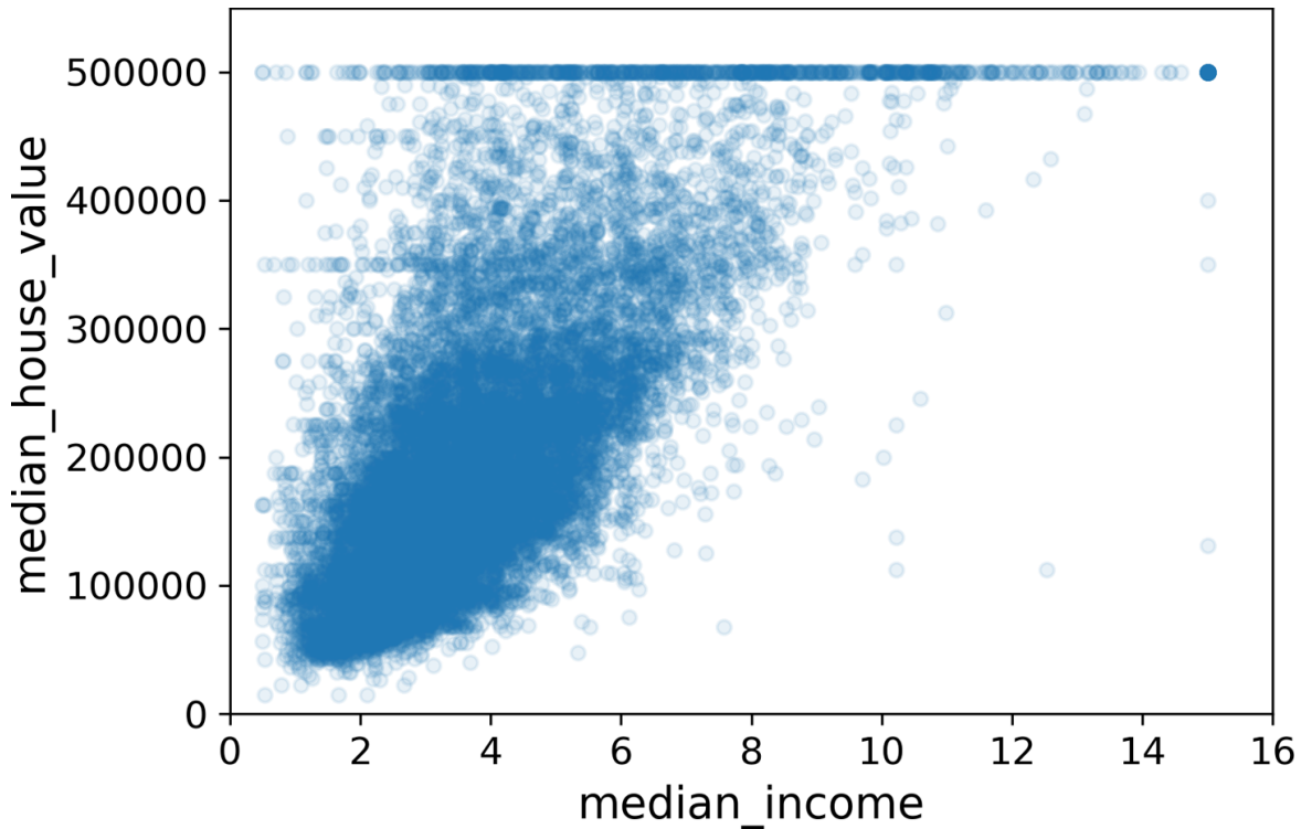
Figure 2-16. Median income versus median house value
