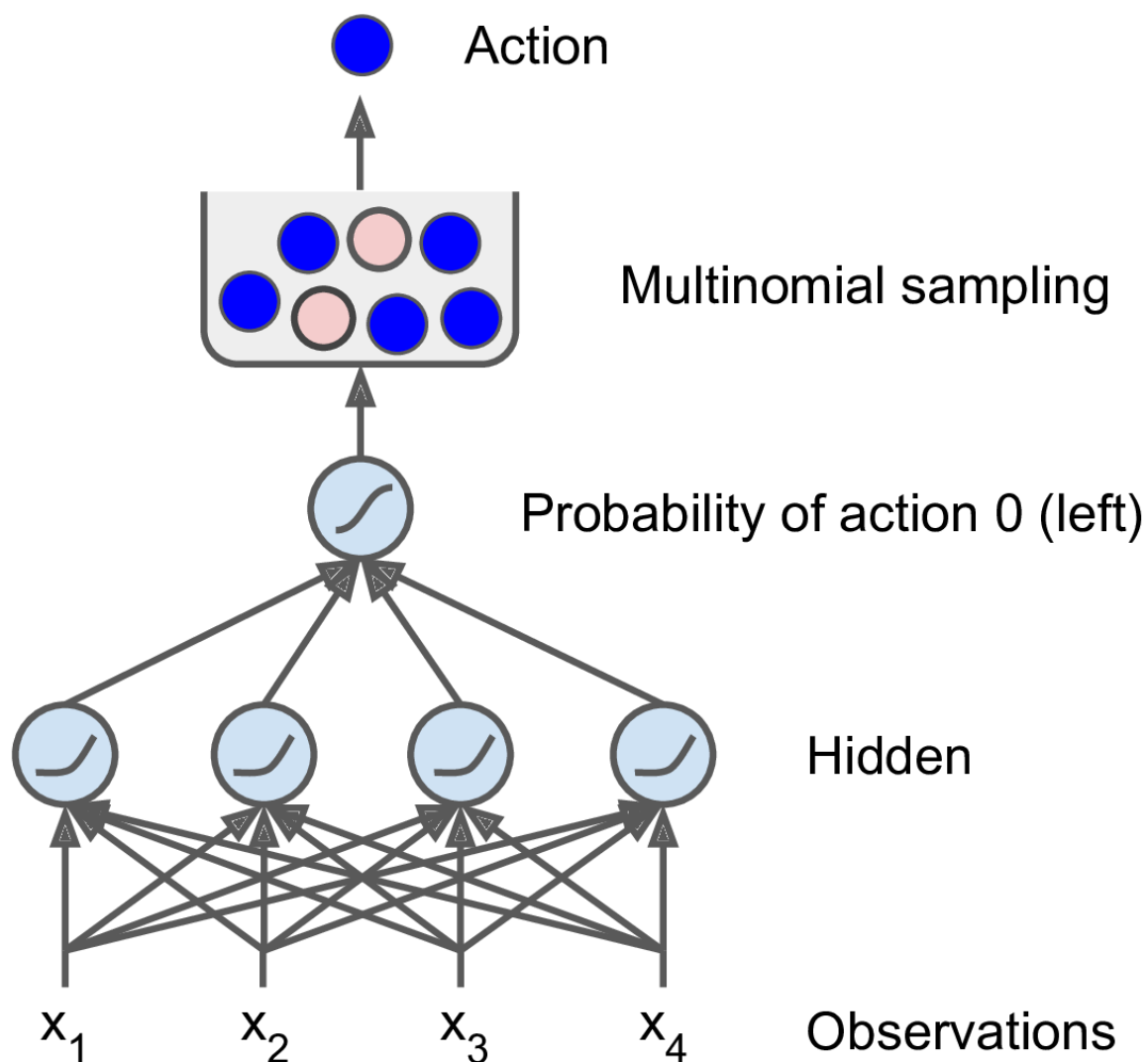
Figure 18-5. Neural network policy
