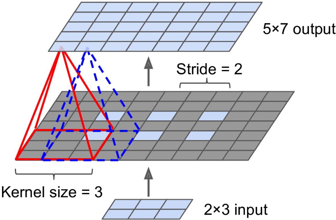
Figure 14-27. Upsampling using a transposed convolutional layer
