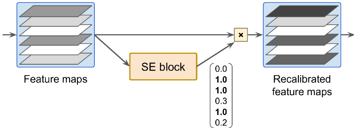
Figure 14-21. An SE block performs feature map recalibration
