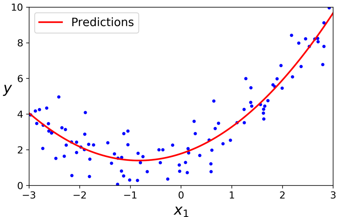
Figure 4-13. Polynomial Regression model predictions
