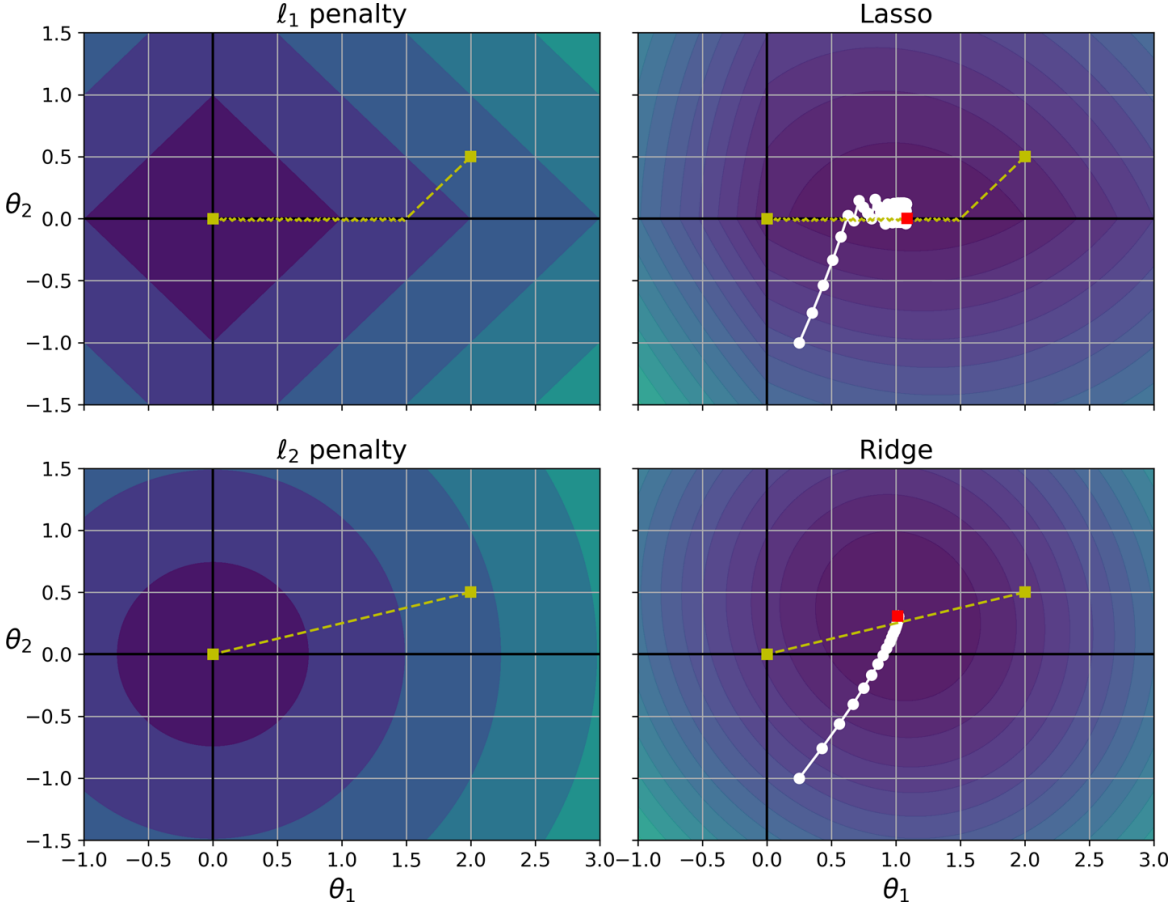
Figure 4-19. Lasso versus Ridge regularization
