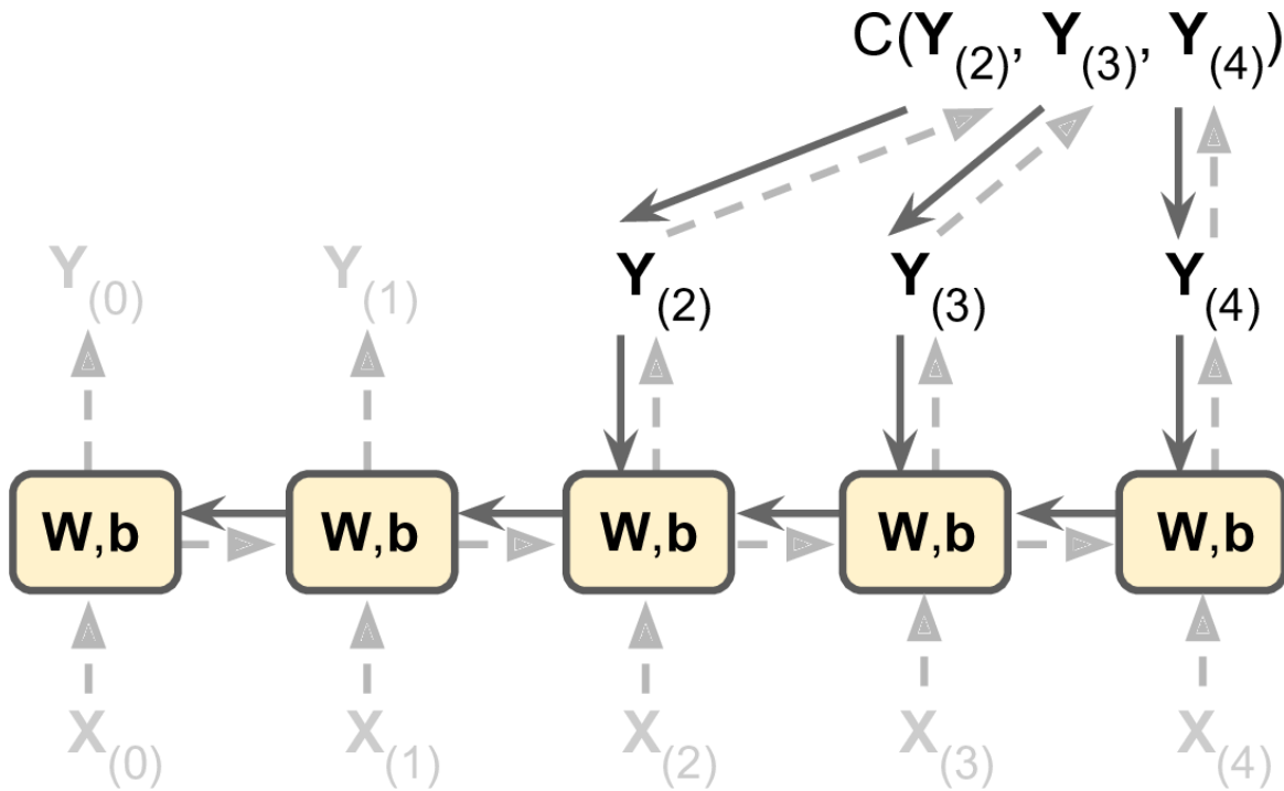
Figure 15-5. Backpropagation through time
