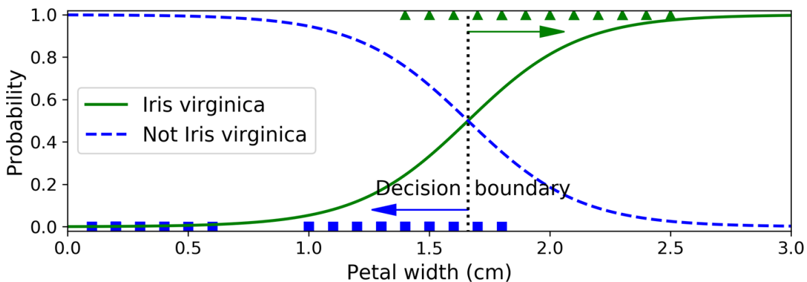
Figure 4-23. Estimated probabilities and decision boundary
