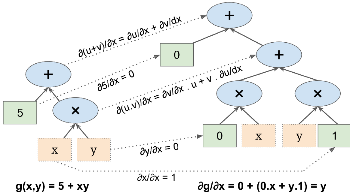
Figure D-1. Forward-mode autodiff
