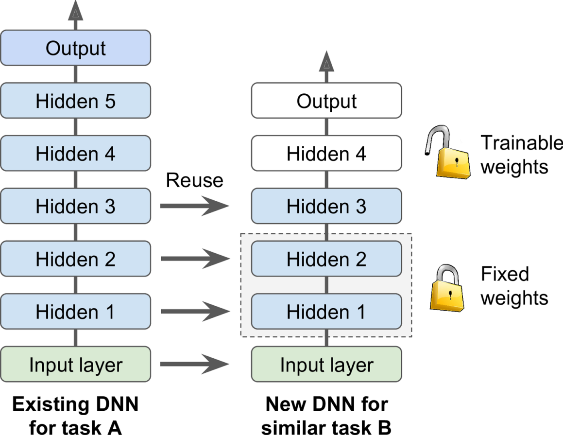
Figure 11-4. Reusing pretrained layers
