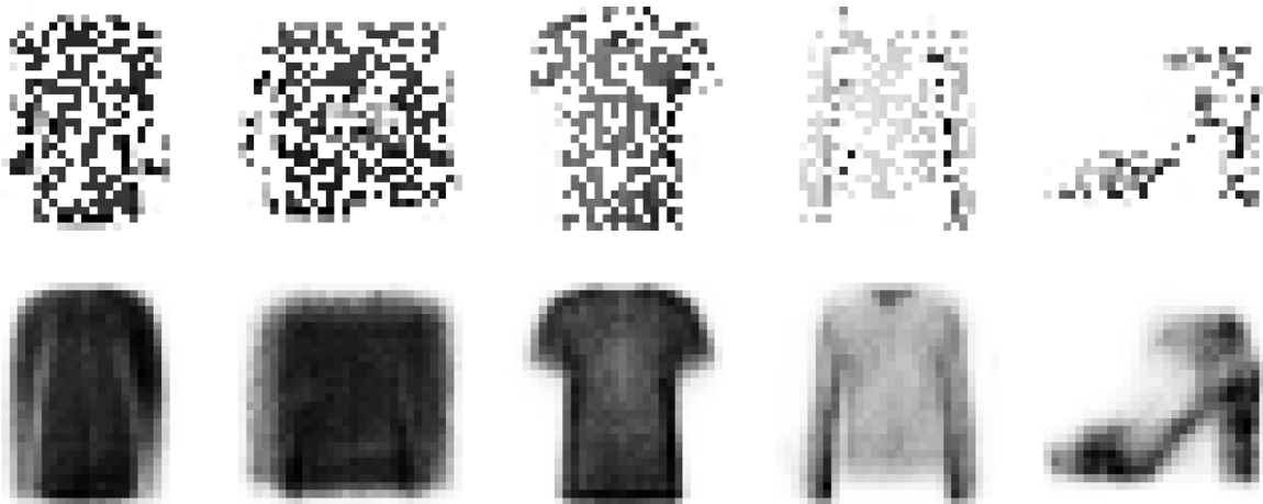
Figure 17-9. Noisy images (top) and their reconstructions (bottom)
