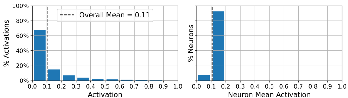
Figure 17-11. Distribution of all the activations in the coding layer (left) and distribution of the mean activation per neuron (right)
