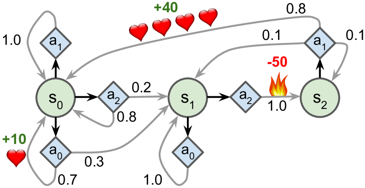
Figure 18-8. Example of a Markov decision process
