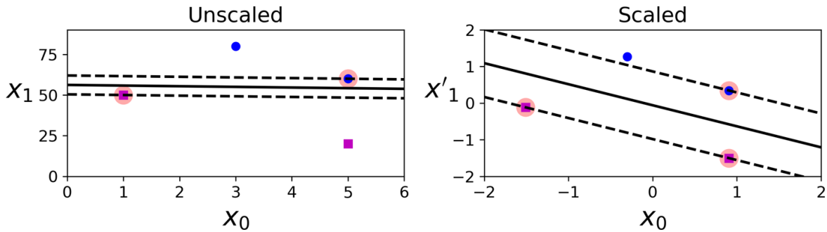
Figure 5-2. Sensitivity to feature scales
