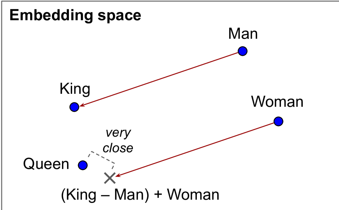
Figure 13-5. Word embeddings of similar words tend to be close, and some axes seem to encode meaningful concepts
