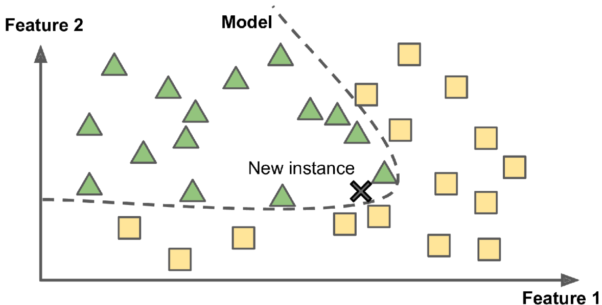
Figure 1-16. Model-based learning
