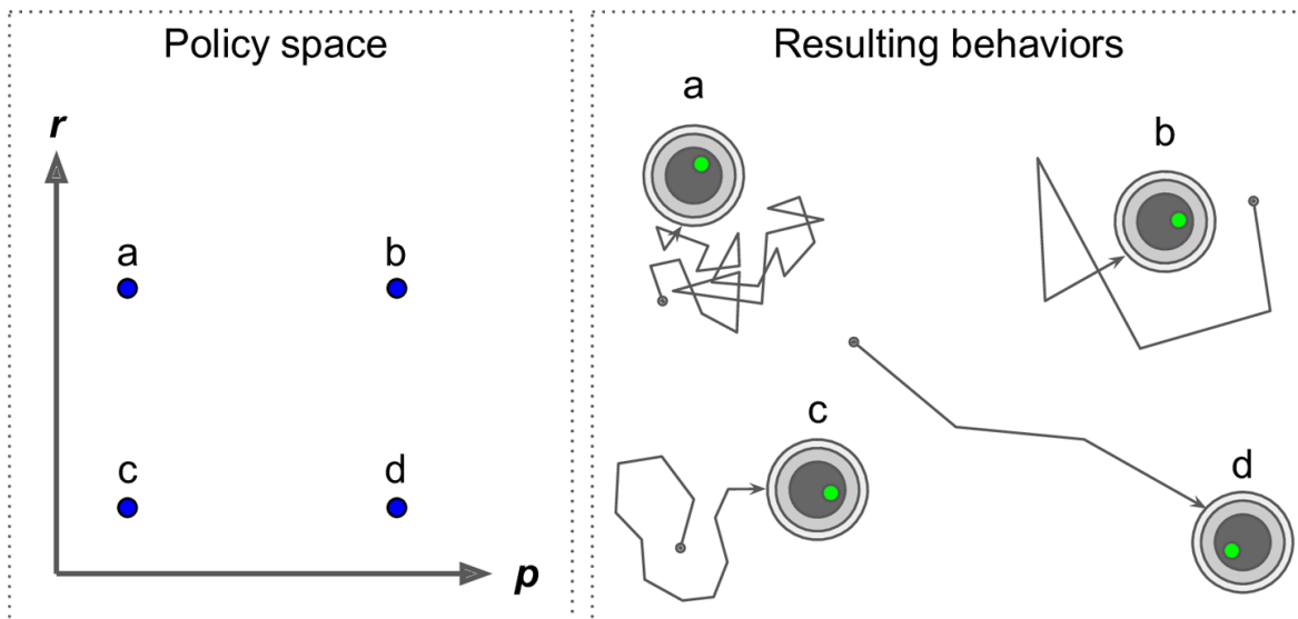
Figure 18-3. Four points in policy space (left) and the agent's corresponding behavior (right)
