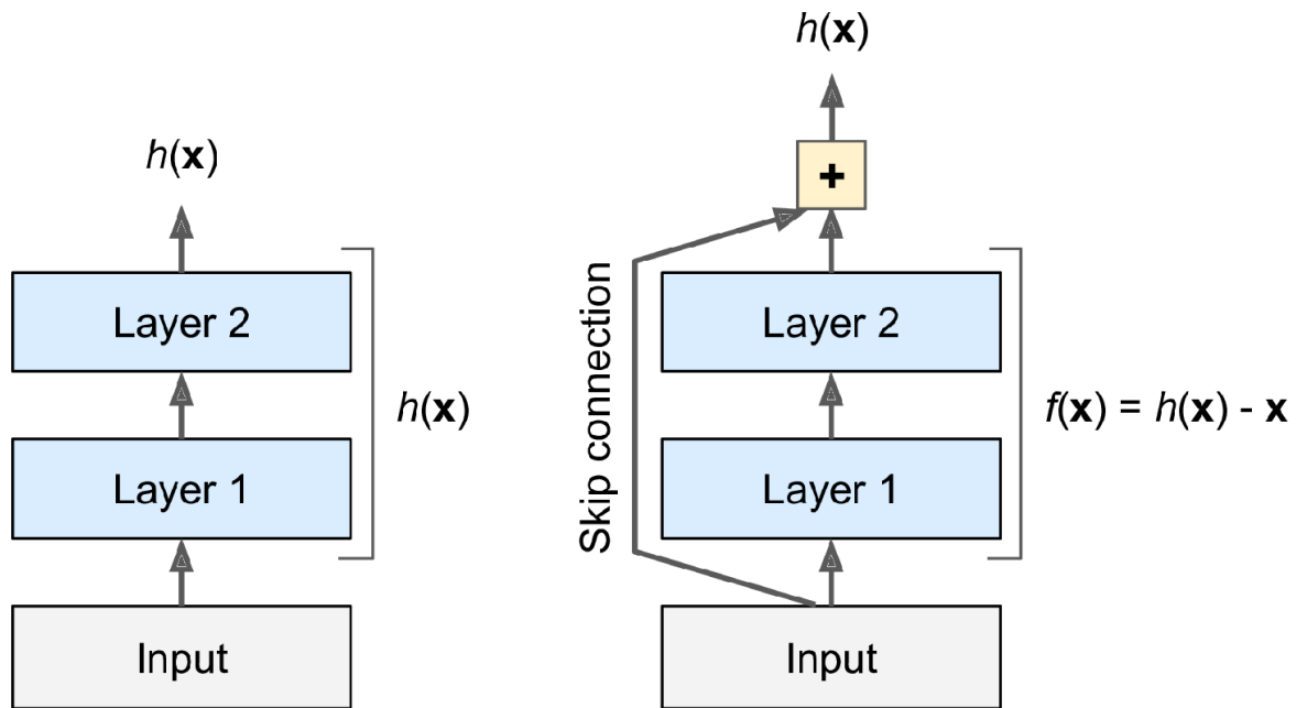
Figure 14-15. Residual learning
