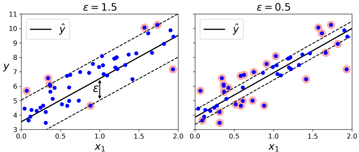
Figure 5-10. SVM Regression
