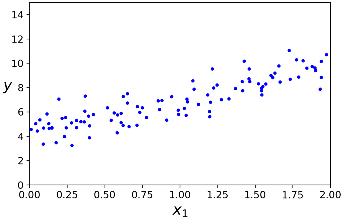
Figure 4-1. Randomly generated linear dataset
