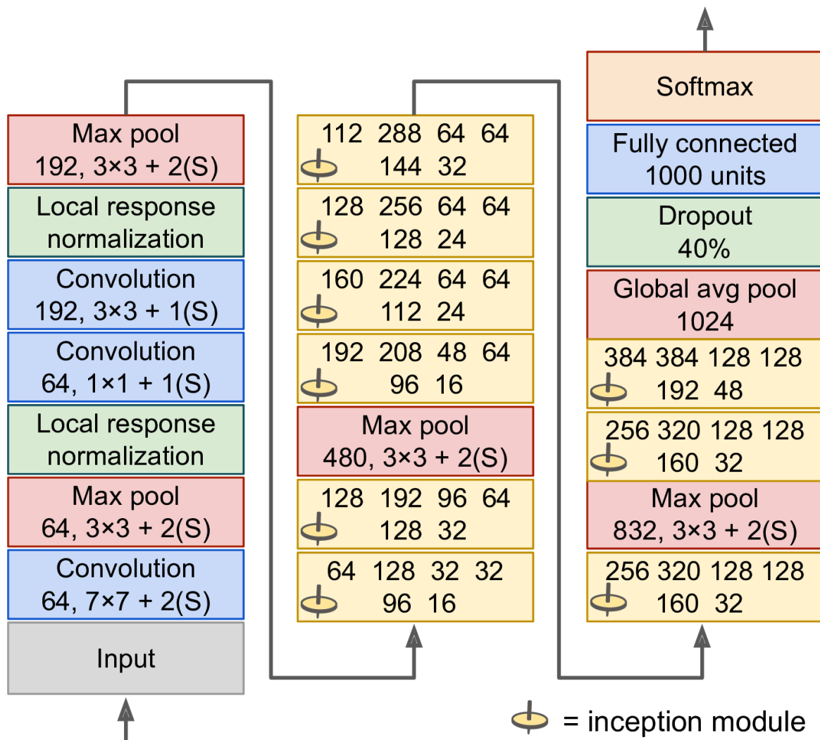
Figure 14-14. GoogLeNet architecture
