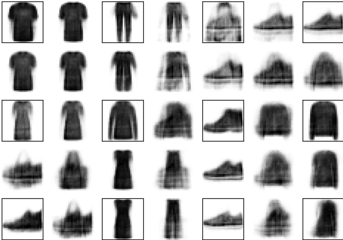
Figure 17-14. Semantic interpolation
