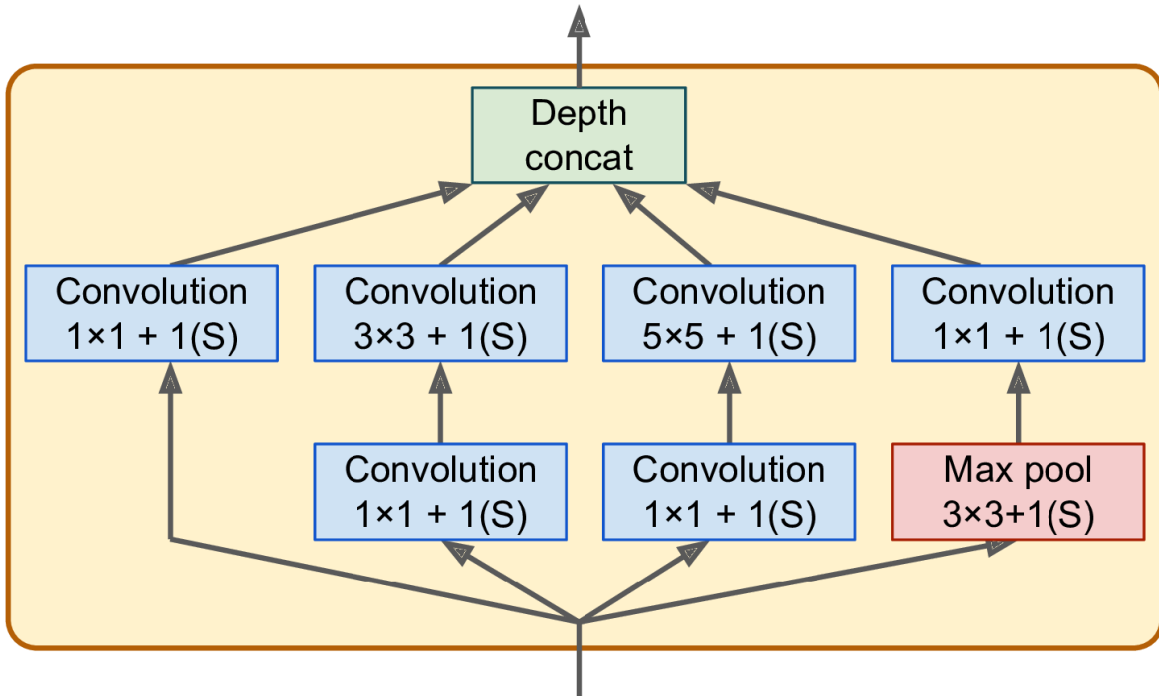
Figure 14-13. Inception module
