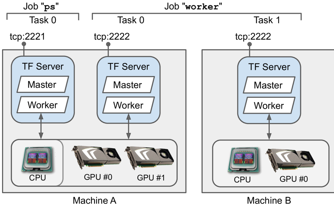
Figure 19-21. TensorFlow cluster
