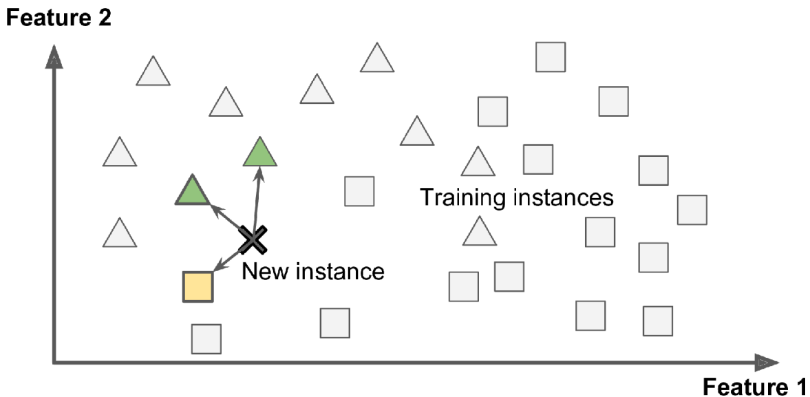
Figure 1-15. Instance-based learning
