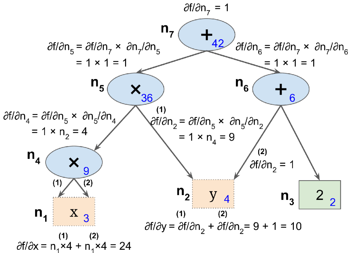
Figure D-3. Reverse-mode autodiff
