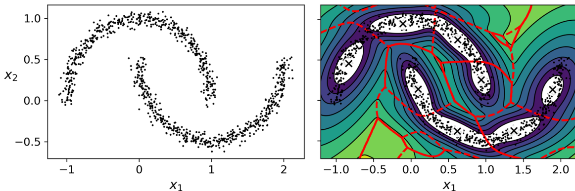
Figure 9-24. Fitting a Gaussian mixture to nonellipsoidal clusters
