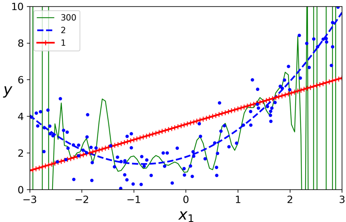
Figure 4-14. High-degree Polynomial Regression
