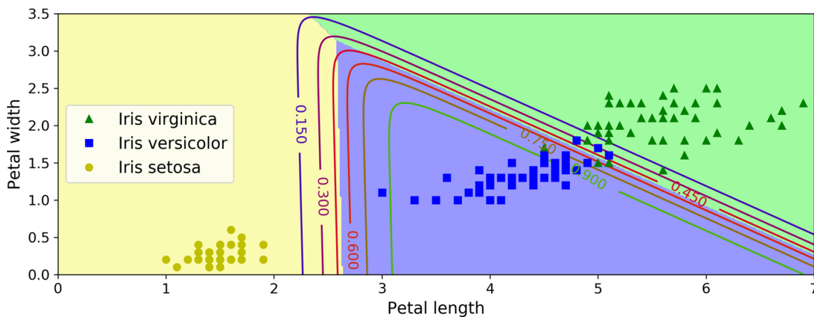
Figure 4-25. Softmax Regression decision boundaries
