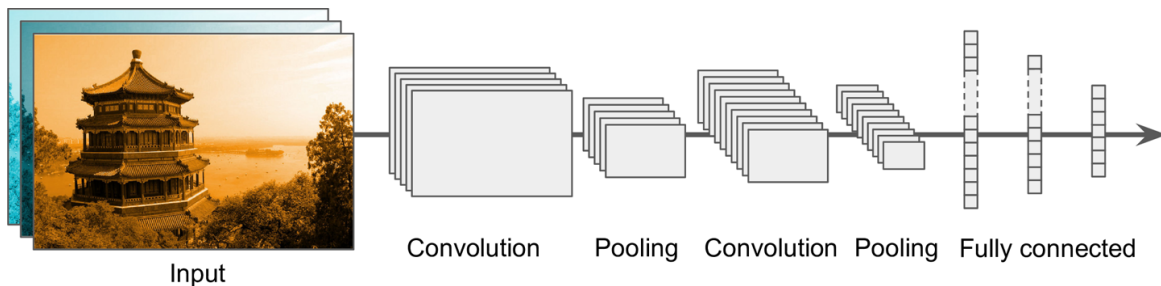
Figure 14-11. Typical CNN architecture
