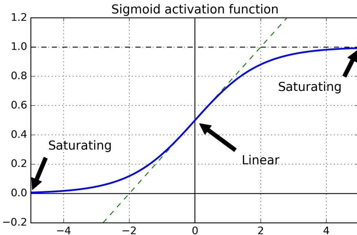
Figure 11-1. Logistic activation function saturation
