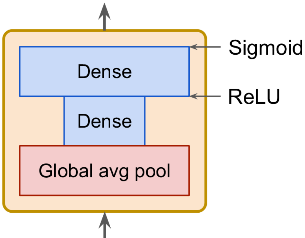
Figure 14-22. SE block architecture
