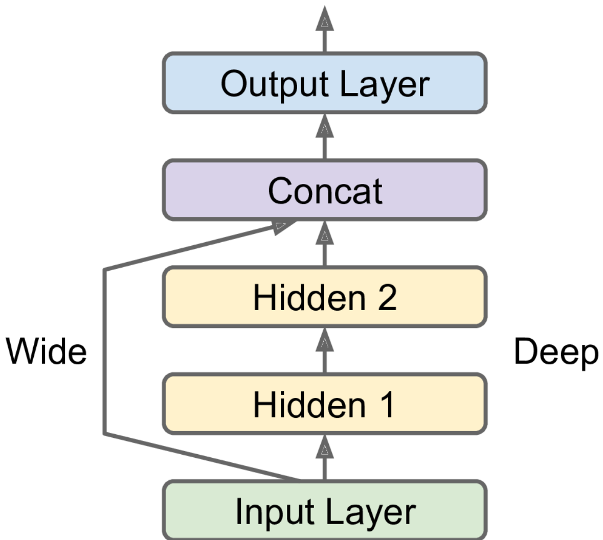
Figure 10-14. Wide & Deep neural network
