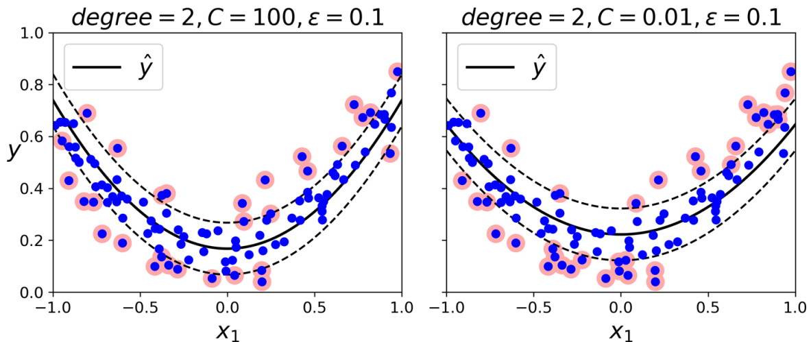
Figure 5-11. SVM Regression using a second-degree polynomial kernel
