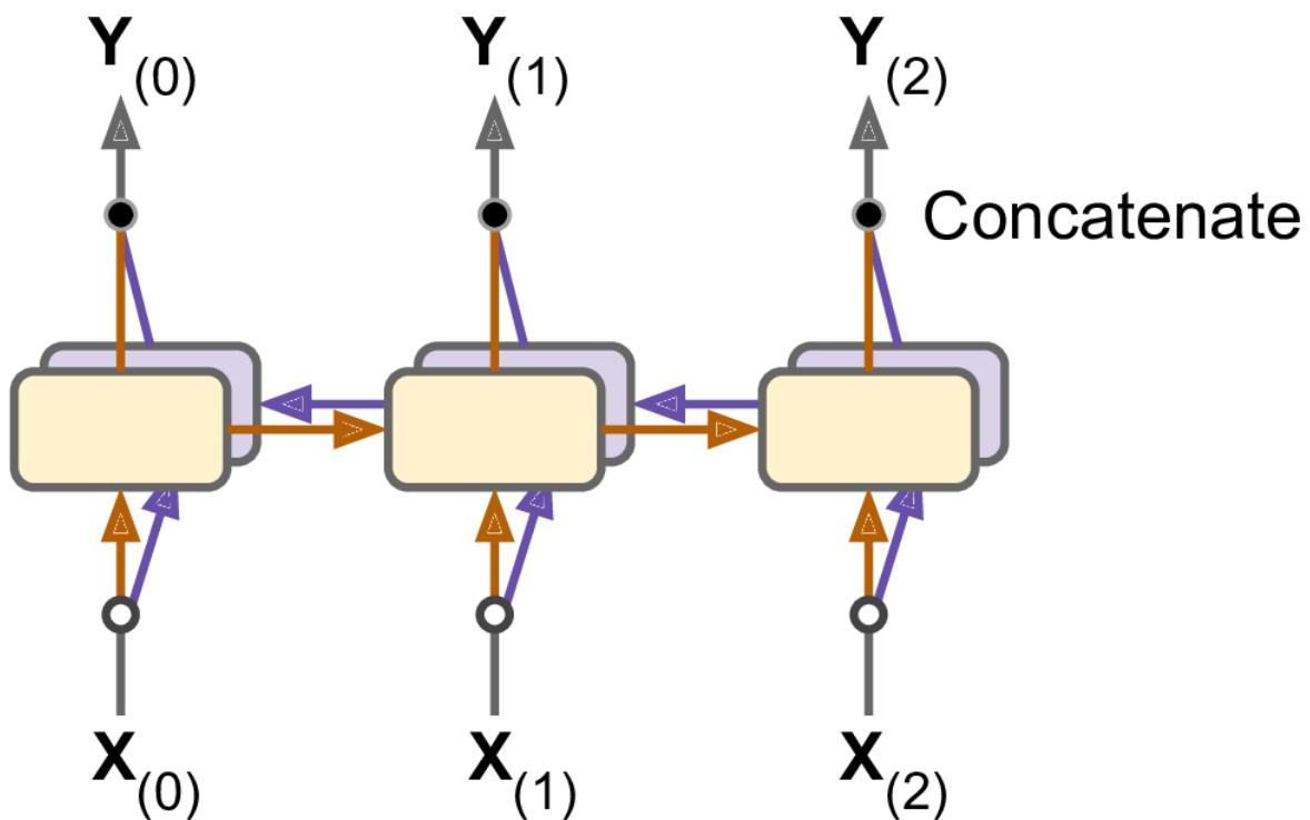
Figure 16-5. A bidirectional recurrent layer
