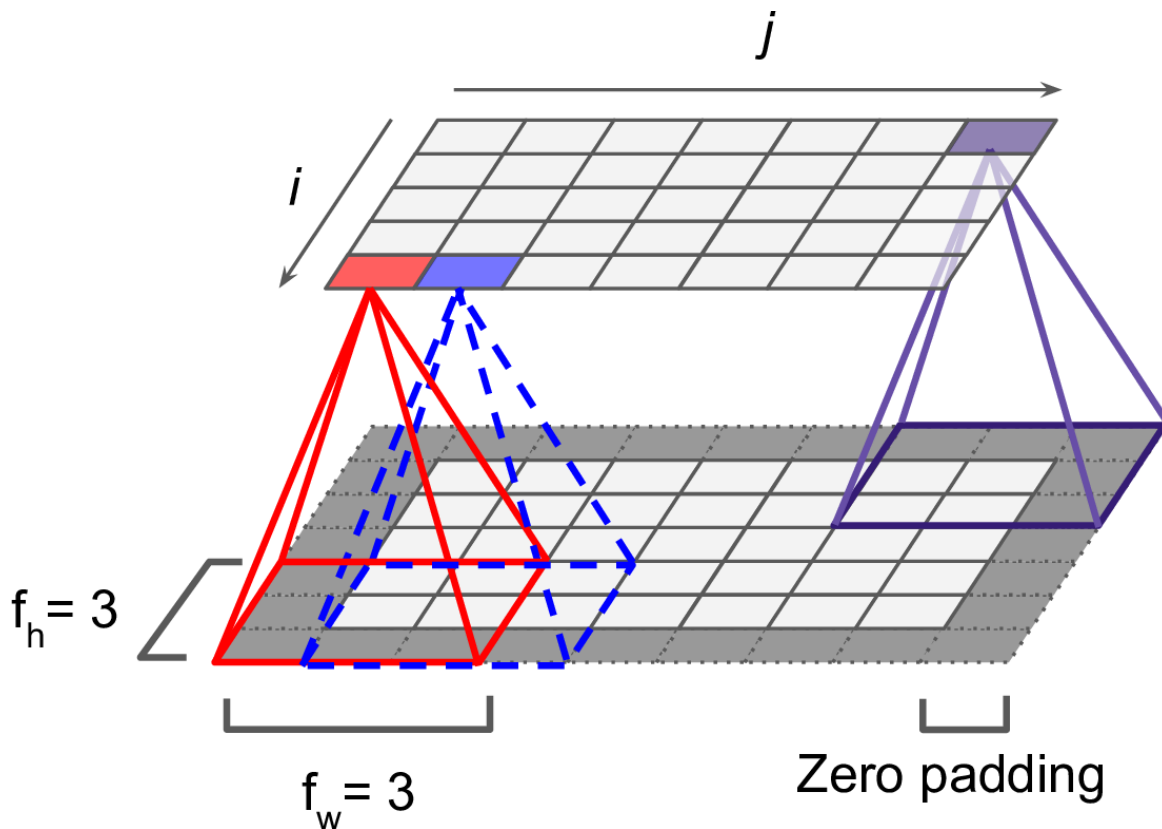
Figure 14-3. Connections between layers and zero padding
