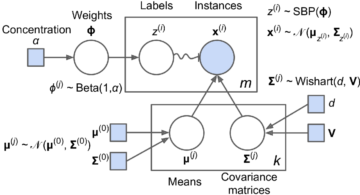
Figure 9-22. Bayesian Gaussian mixture model
