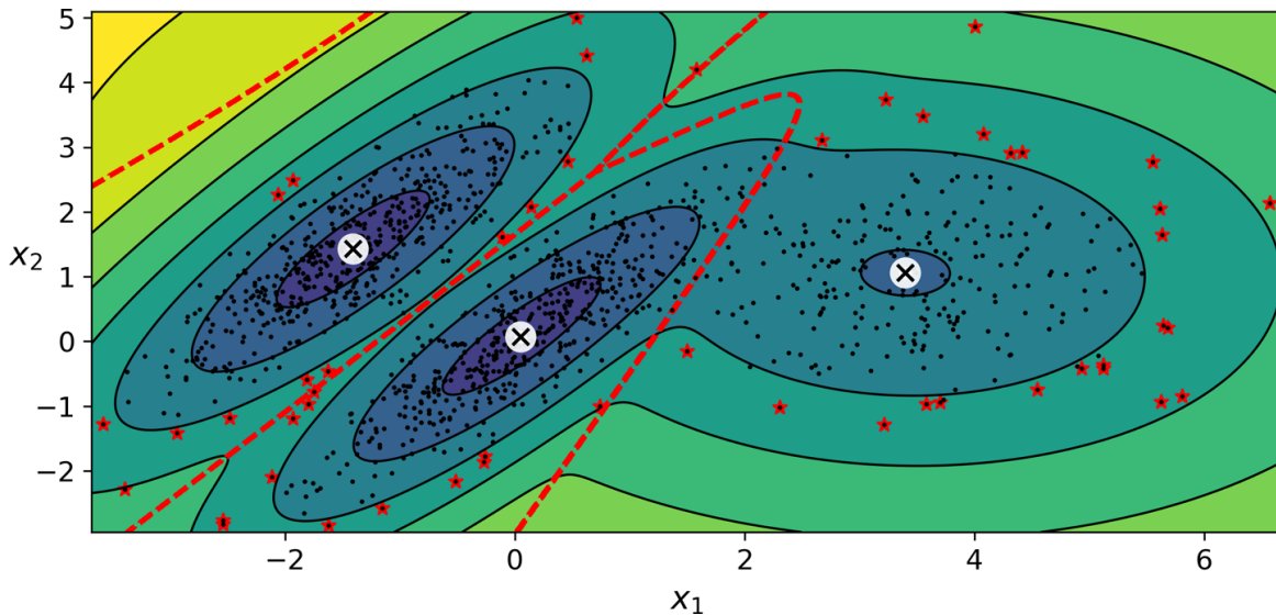
Figure 9-19. Anomaly detection using a Gaussian mixture model
