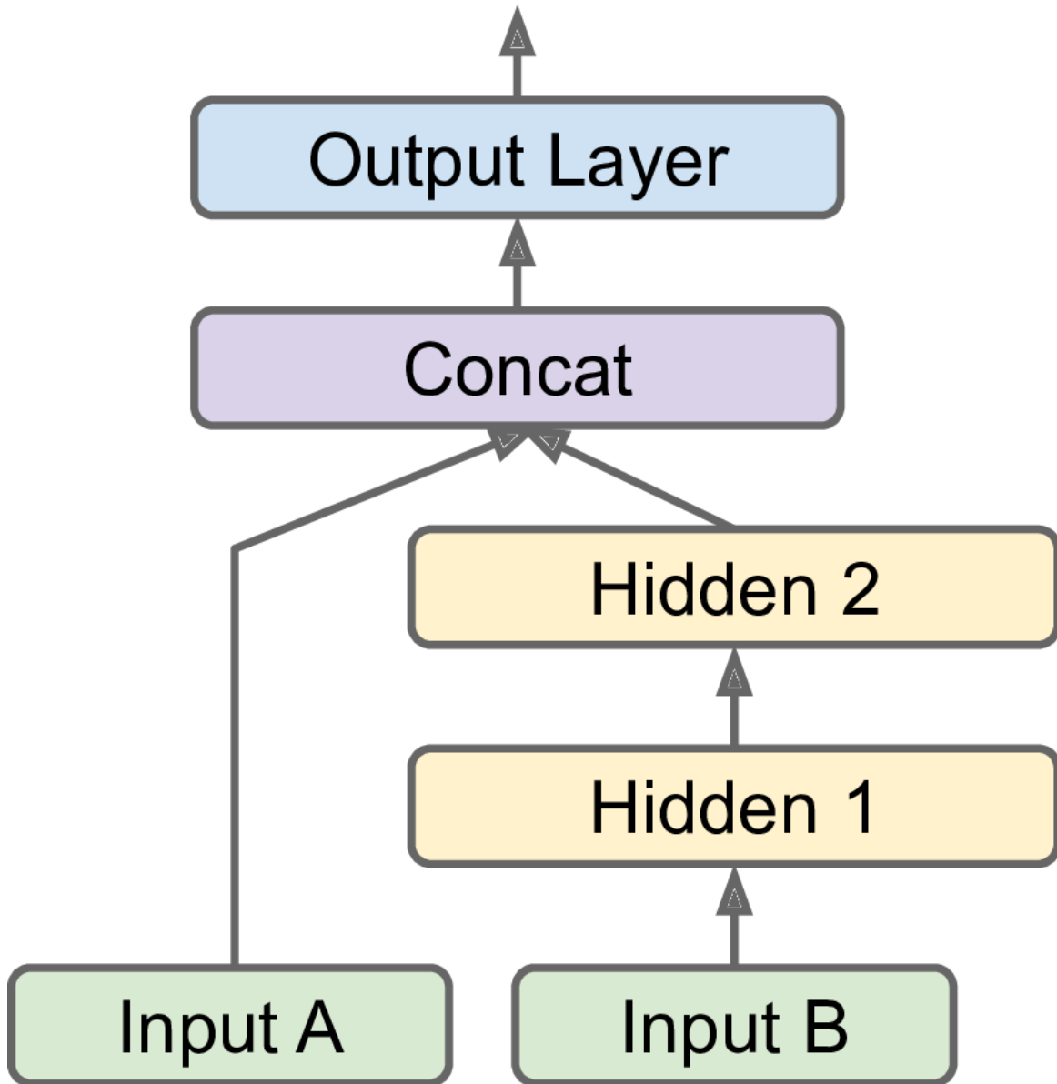
Figure 10-15. Handling multiple inputs
