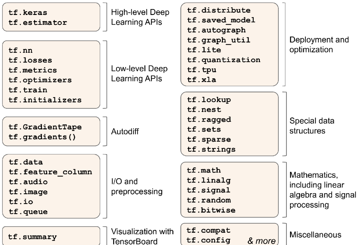
Figure 12-1. TensorFlow’s Python API
