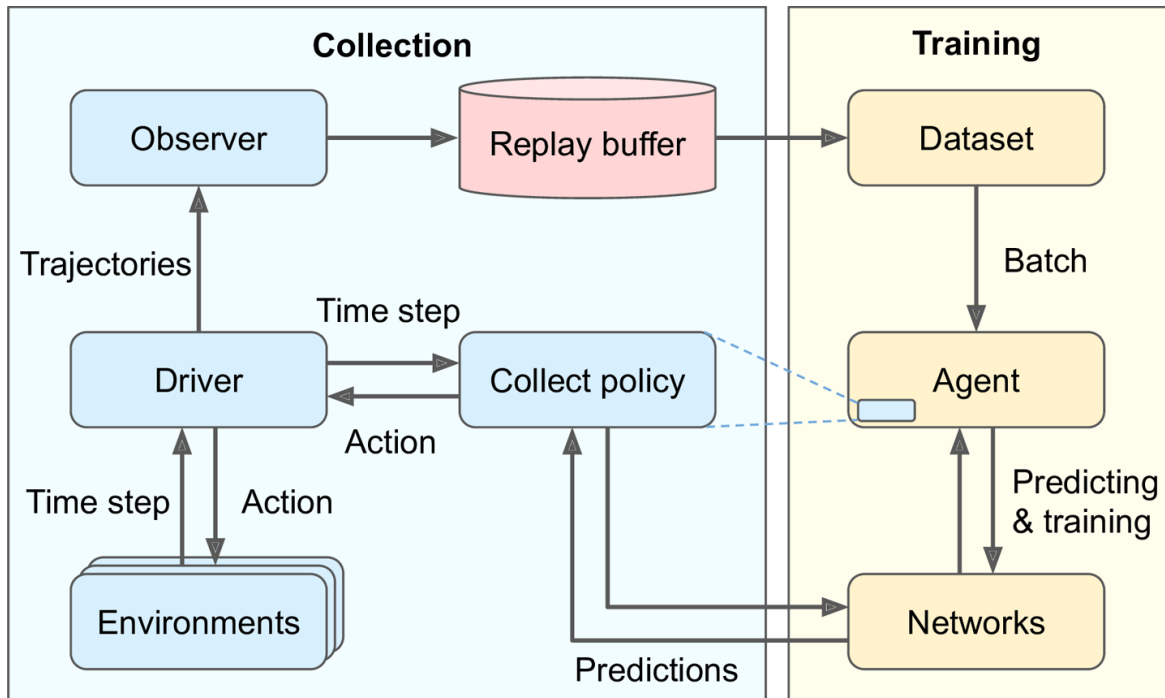
Figure 18-13. A typical TF-Agents training architecture
