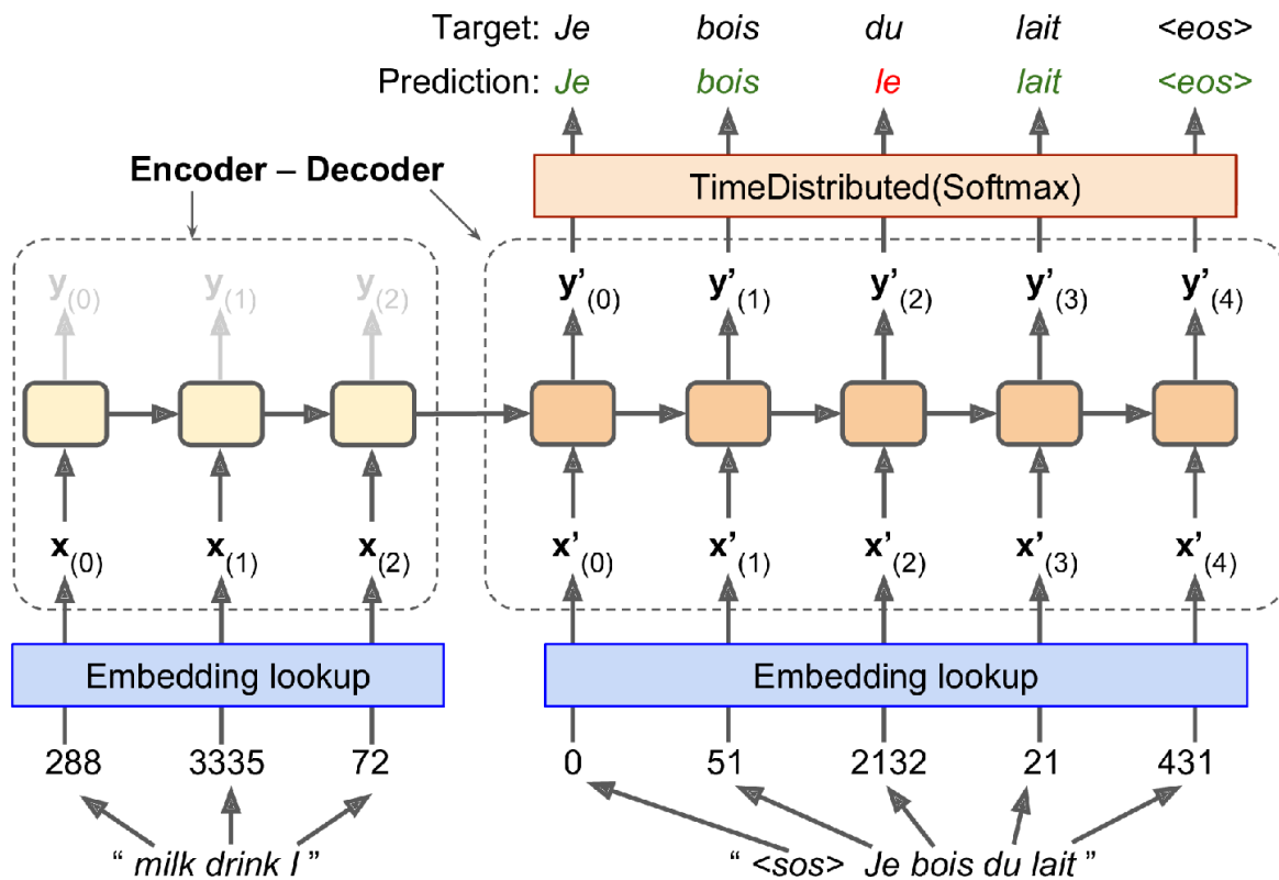
Figure 16-3. A simple machine translation model
