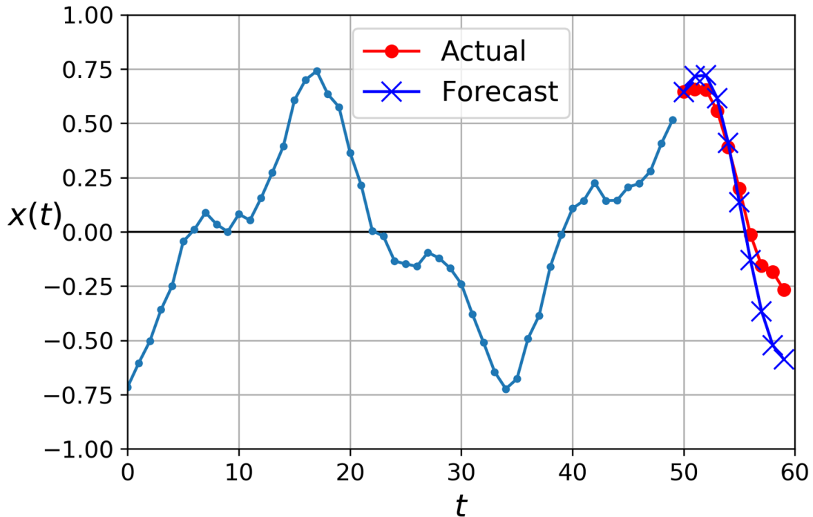
Figure 15-8. Forecasting 10 steps ahead, 1 step at a time
