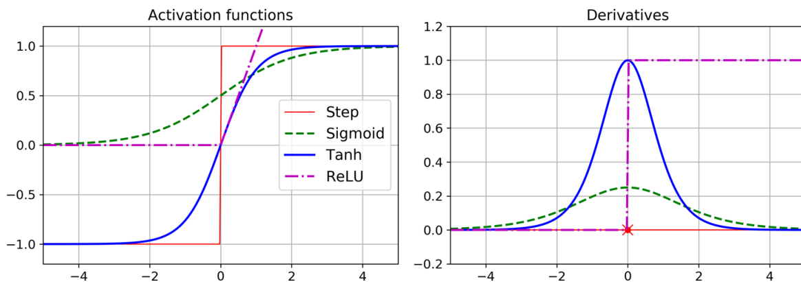
Figure 10-8. Activation functions and their derivatives
