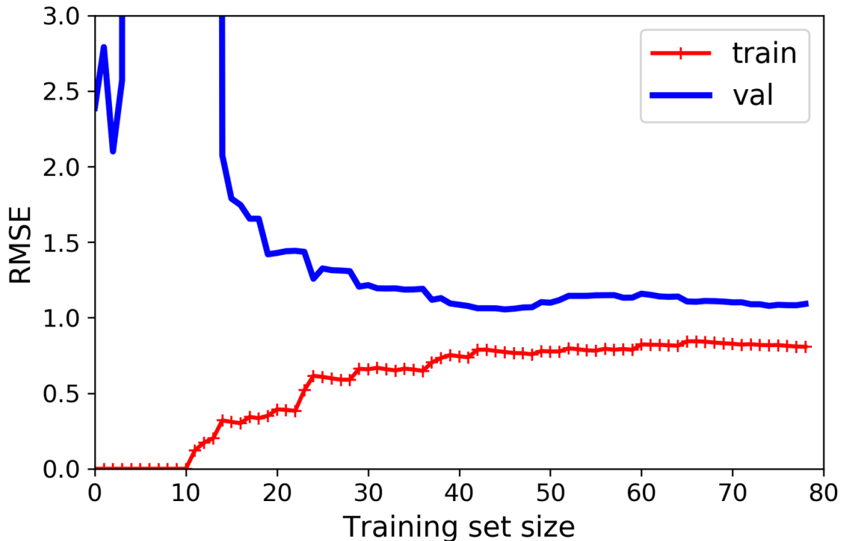
Figure 4-16. Learning curves for the 10th-degree polynomial model
