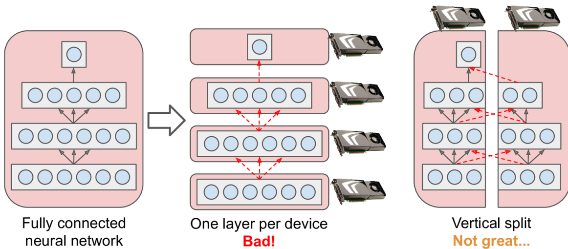
Figure 19-15. Splitting a fully connected neural network
