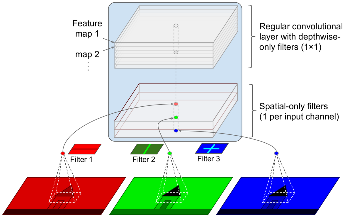
Figure 14-19. Depthwise separable convolutional layer
