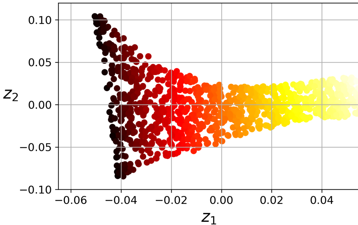
Figure 8-12. Unrolled Swiss roll using LLE
