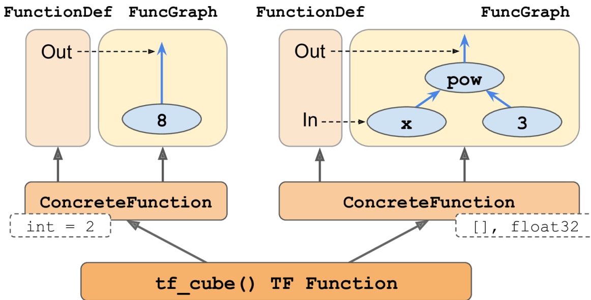
Figure G-1. The tf_cube() TF Function, with its ConcreteFunction s and their FuncGraph s
