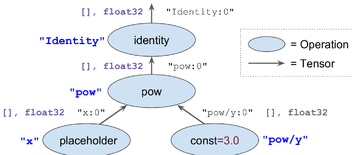
Figure G-2. Example of a computation graph
