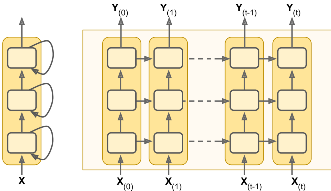
Figure 15-7. Deep RNN (left) unrolled through time (right)
