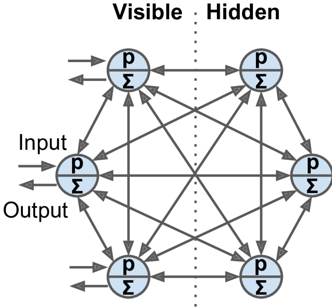
Figure E-2. Boltzmann machine
