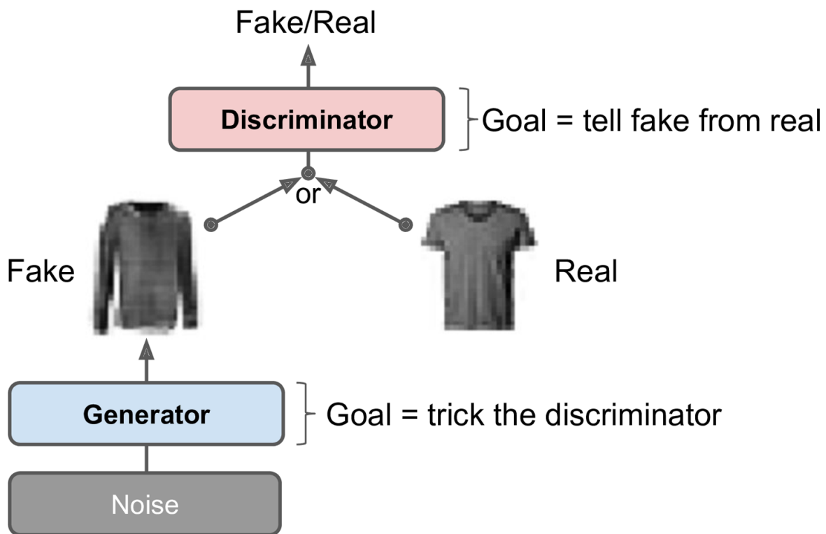
Figure 17-15. A generative adversarial network
