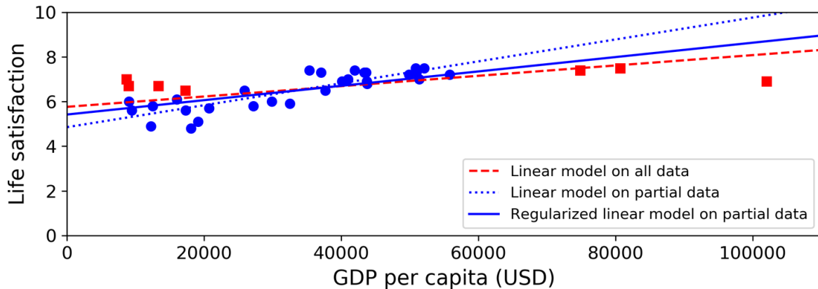
Figure 1-23. Regularization reduces the risk of overfitting
