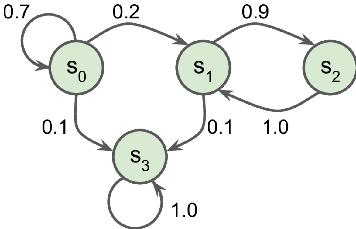
Figure 18-7. Example of a Markov chain
