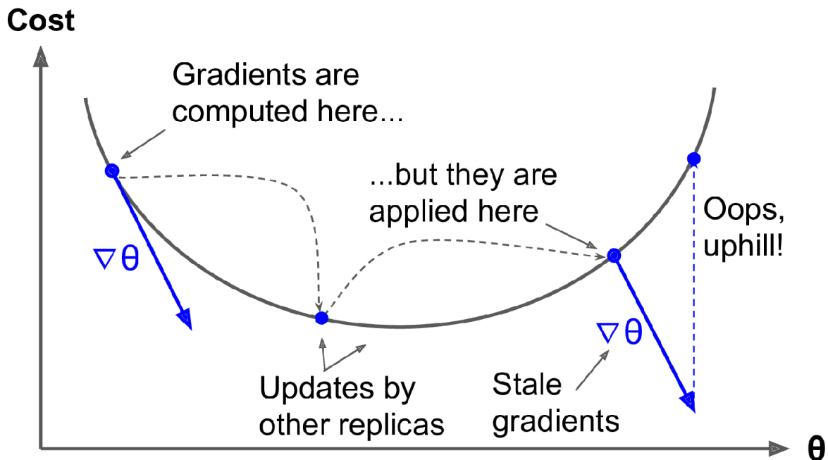
Figure 19-20. Stale gradients when using asynchronous updates
