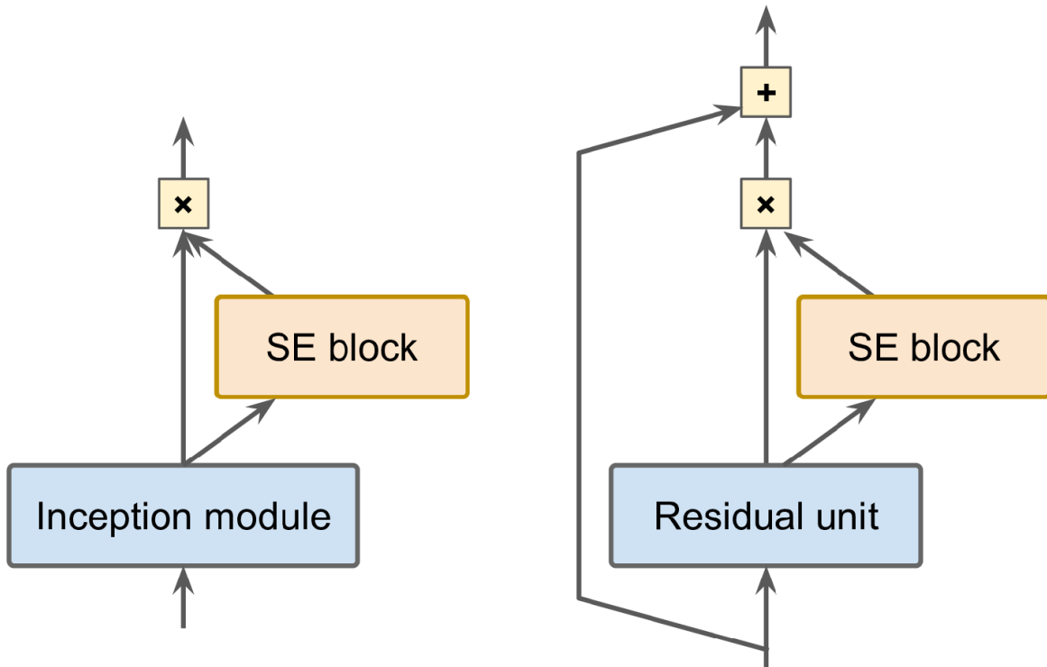
Figure 14-20. SE-Inception module (left) and SE-ResNet unit (right)
