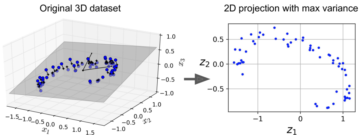
Figure 17-2. PCA performed by an undercomplete linear autoencoder
