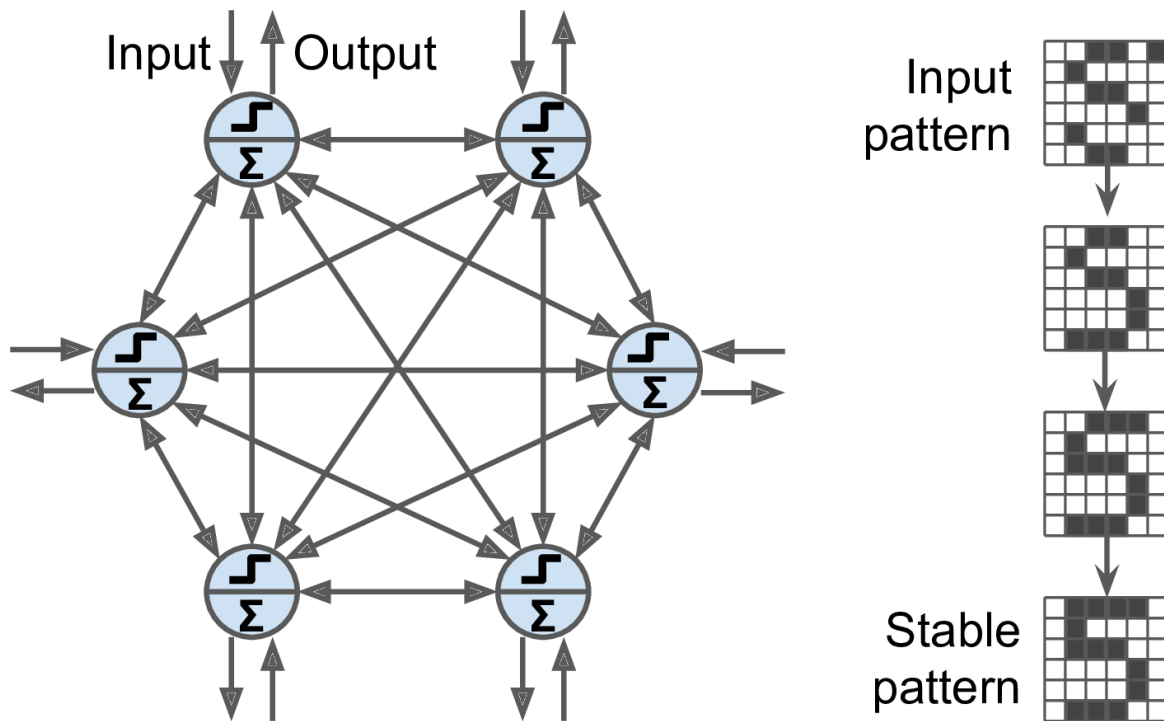
Figure E-1. Hopfield network
