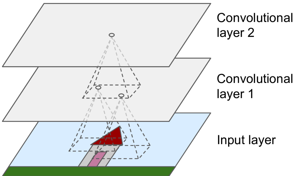
Figure 14-2. CNN layers with rectangular local receptive fields
