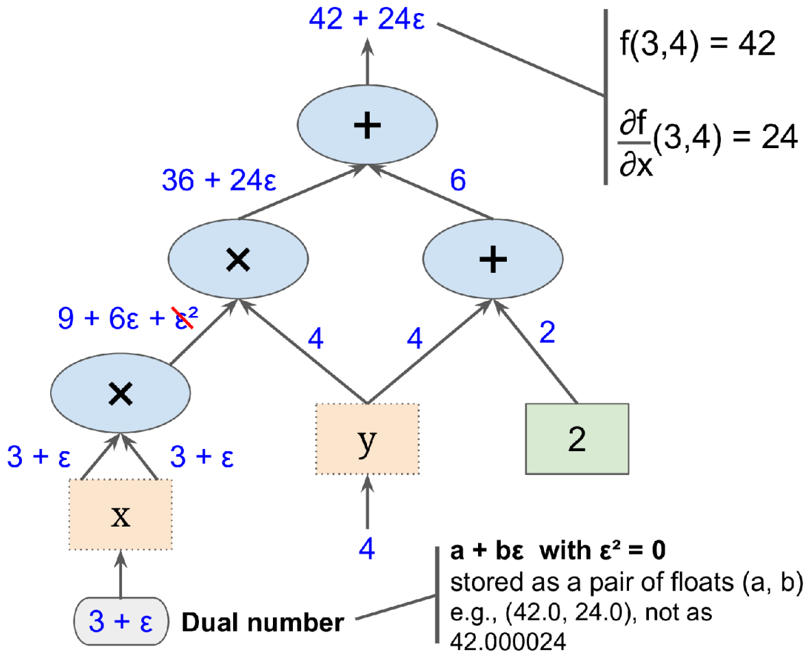
Figure D-2. Forward-mode autodiff using dual numbers
