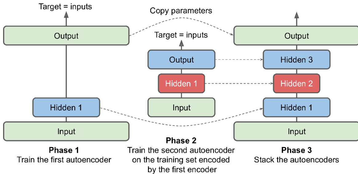
Figure 17-7. Training one autoencoder at a time
