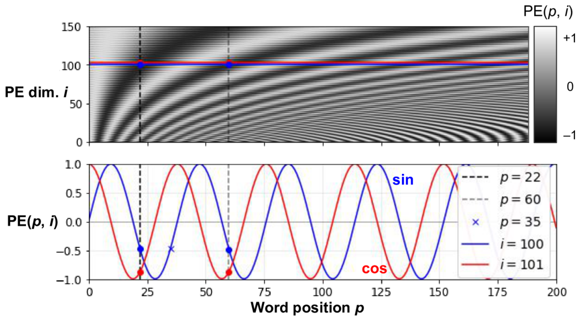
Figure 16-9. Sine/cosine positional embedding matrix (transposed, top) with a focus on two values of i (bottom)
