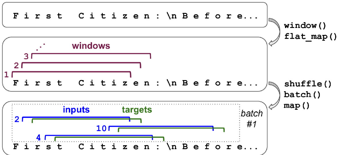
Figure 16-1. Preparing a dataset of shuffled windows
