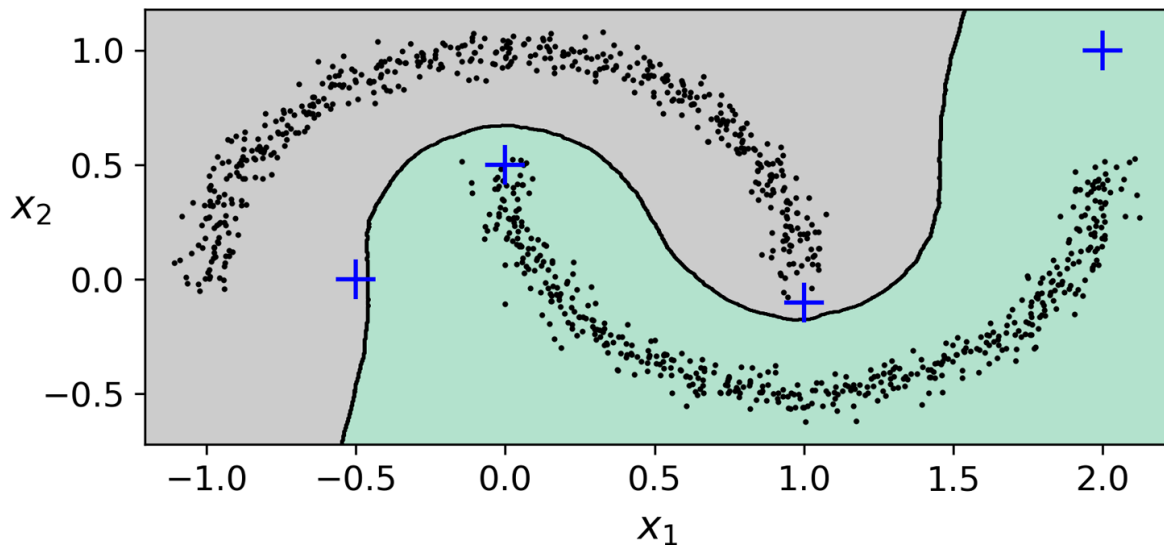
Figure 9-15. Decision boundary between two clusters
