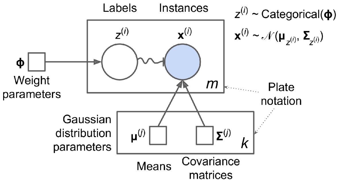
Figure 9-16. A graphical representation of a Gaussian mixture model, including its parameters (squares), random variables (circles), and their conditional dependencies (solid arrows)
