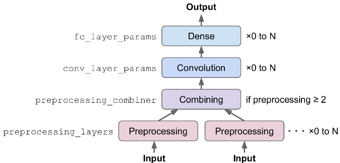
Figure 18-14. Architecture of an encoding network
