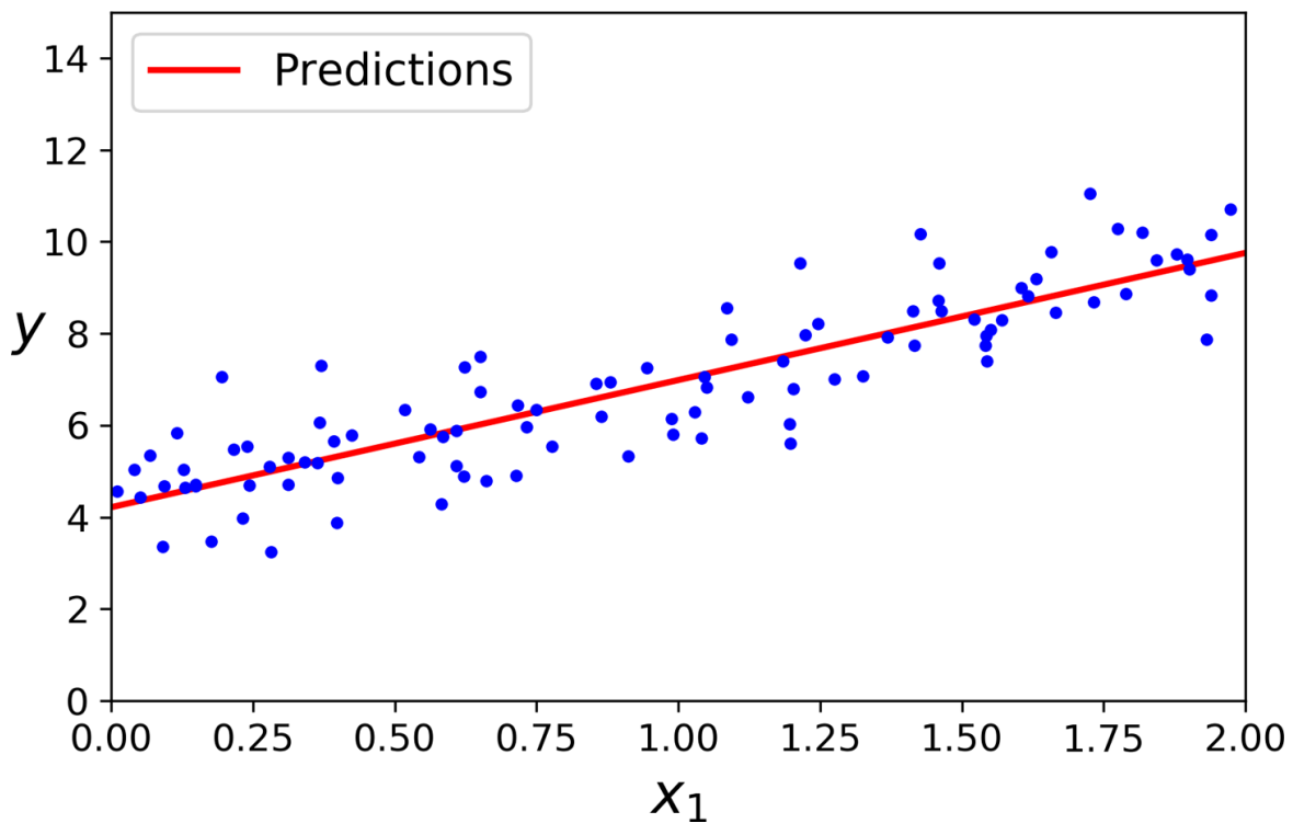
Figure 4-2. Linear Regression model predictions
