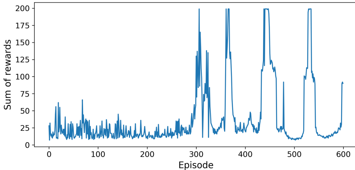
Figure 18-10. Learning curve of the Deep Q-Learning algorithm
