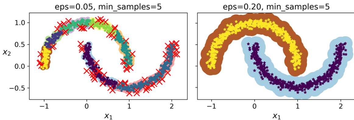
Figure 9-14. DBSCAN clustering using two different neighborhood radiuses
