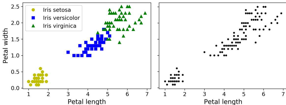
Figure 9-1. Classification (left) versus clustering (right)
