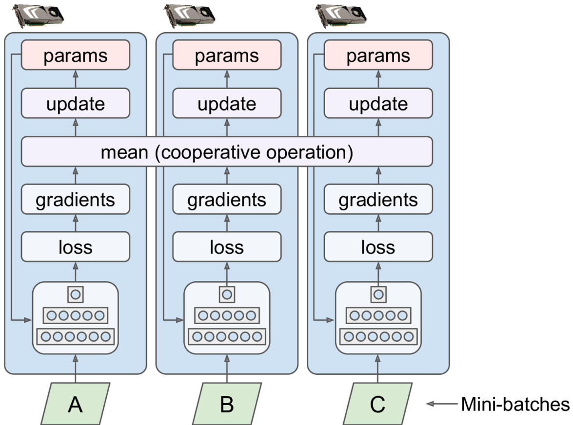
Figure 19-18. Data parallelism using the mirrored strategy
