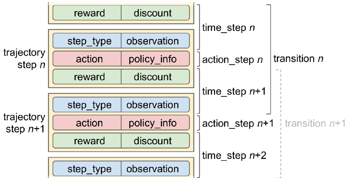
Figure 18-16. Trajectories, transitions, time steps, and action steps
