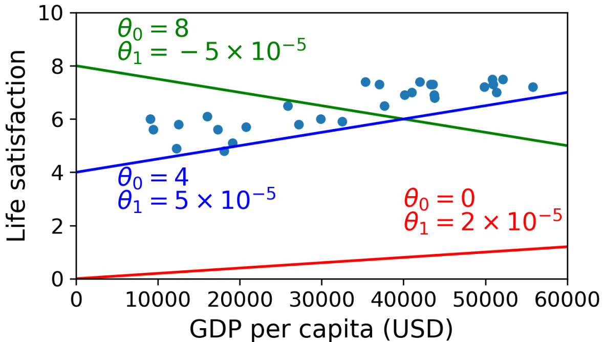
Figure 1-18. A few possible linear models
