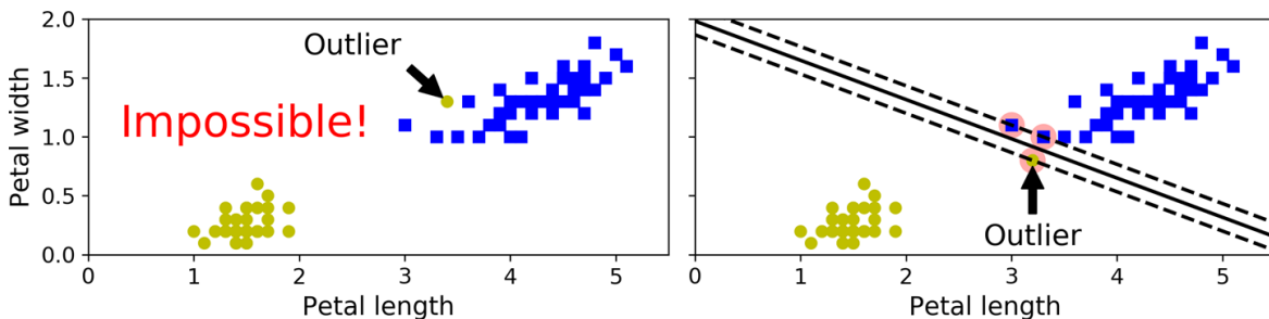
Figure 5-3. Hard margin sensitivity to outliers
