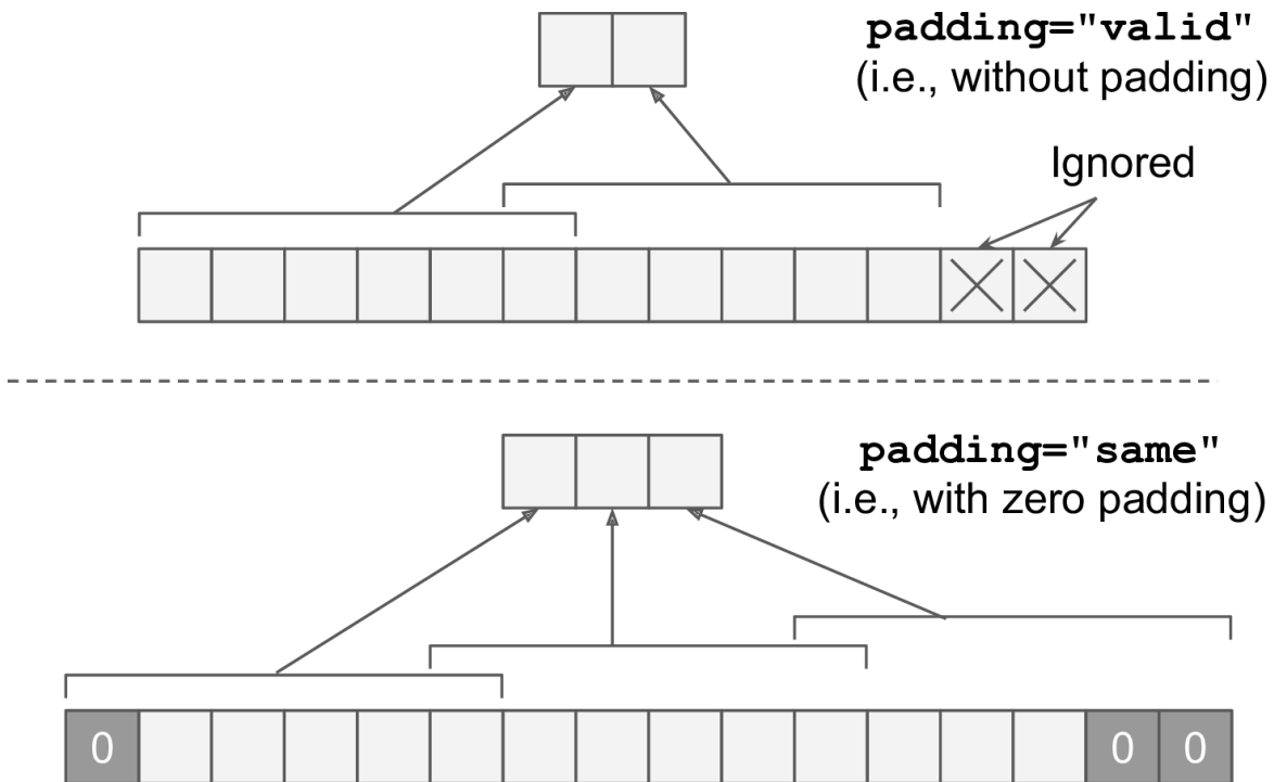
Figure 14-7. Padding="same" or "valid" (with input width 13, filter width 6, stride 5)
