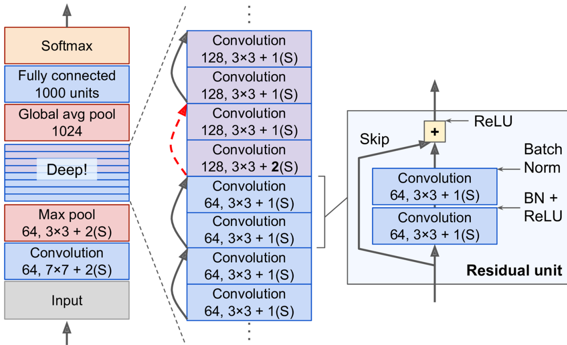
Figure 14-17. ResNet architecture
