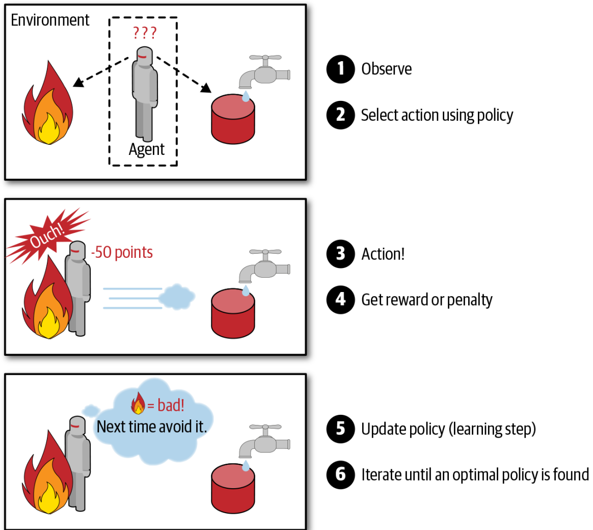
Figure 1-12. Reinforcement Learning
