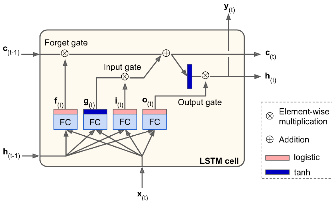
Figure 15-9. LSTM cell
