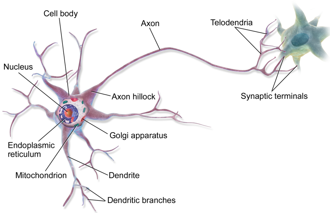
Figure 10-1. Biological neuron 4
