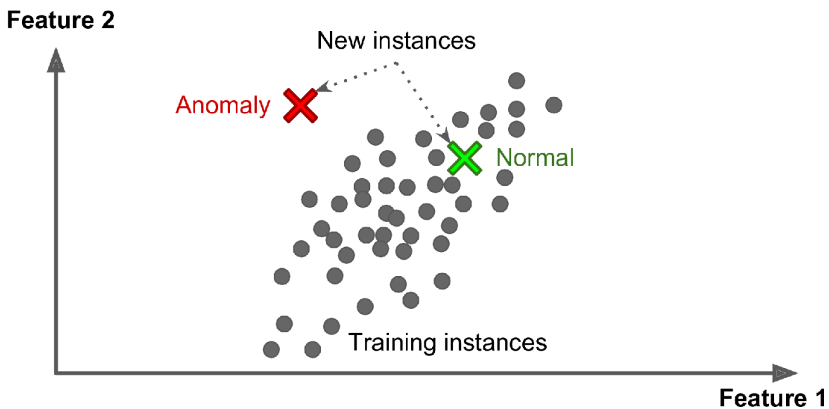
Figure 1-10. Anomaly detection
