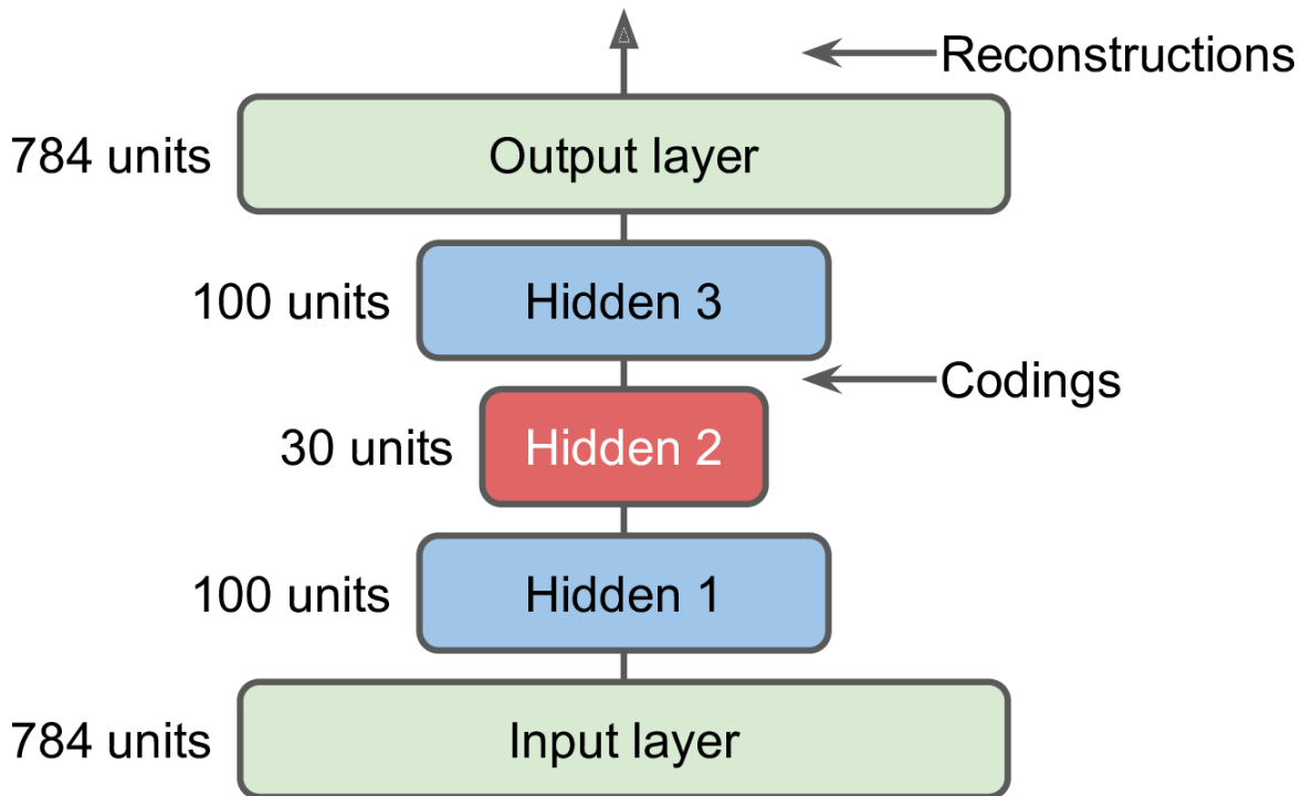
Figure 17-3. Stacked autoencoder
