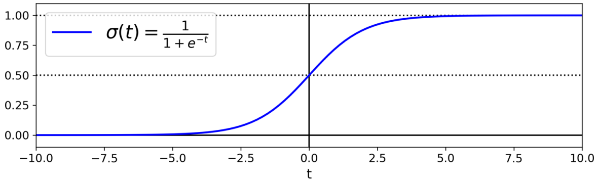
Figure 4-21. Logistic function
