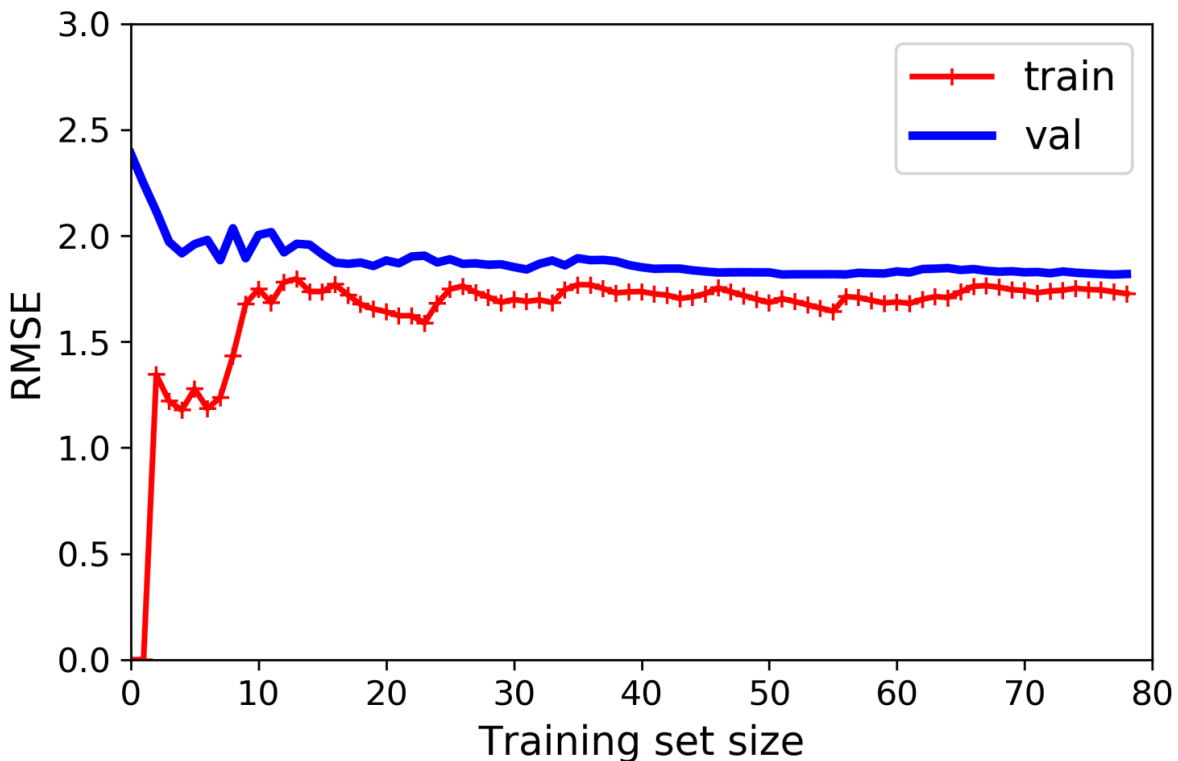
Figure 4-15. Learning curves
