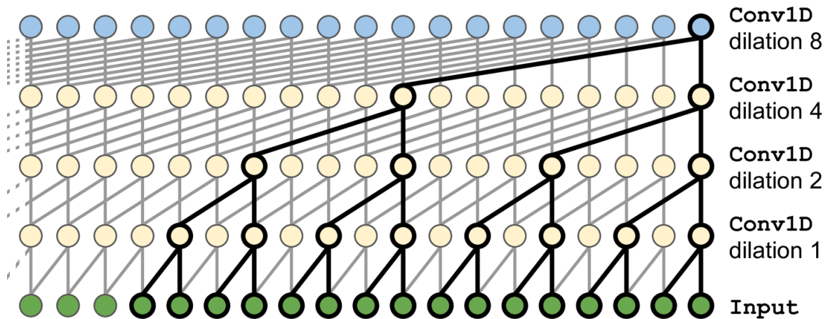
Figure 15-11. WaveNet architecture
