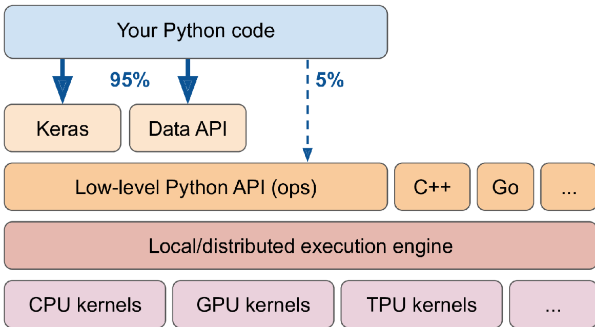
Figure 12-2. TensorFlow's architecture
