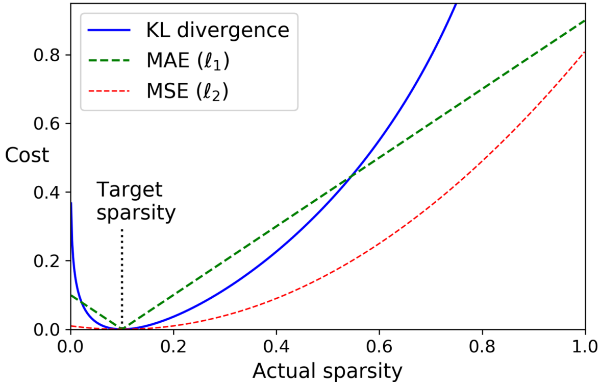
Figure 17-10. Sparsity loss
