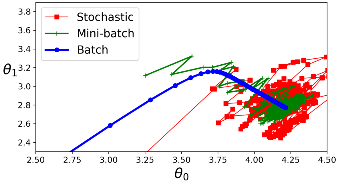
Figure 4-11. Gradient Descent paths in parameter space
