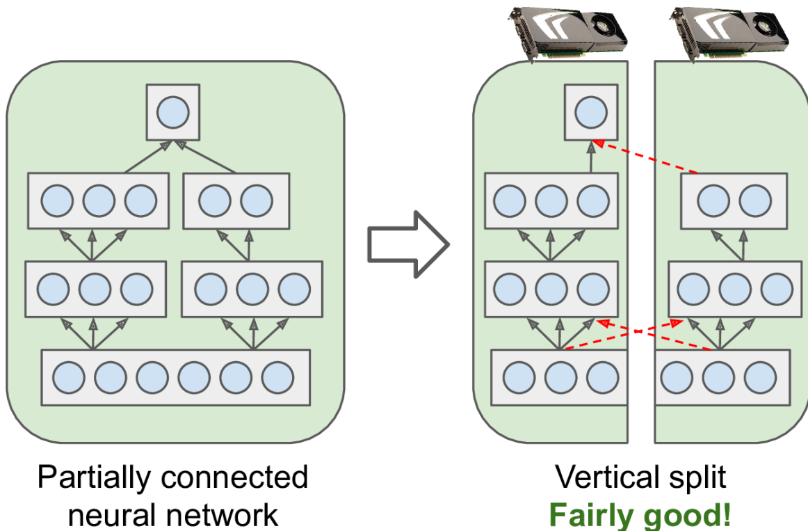
Figure 19-16. Splitting a partially connected neural network
