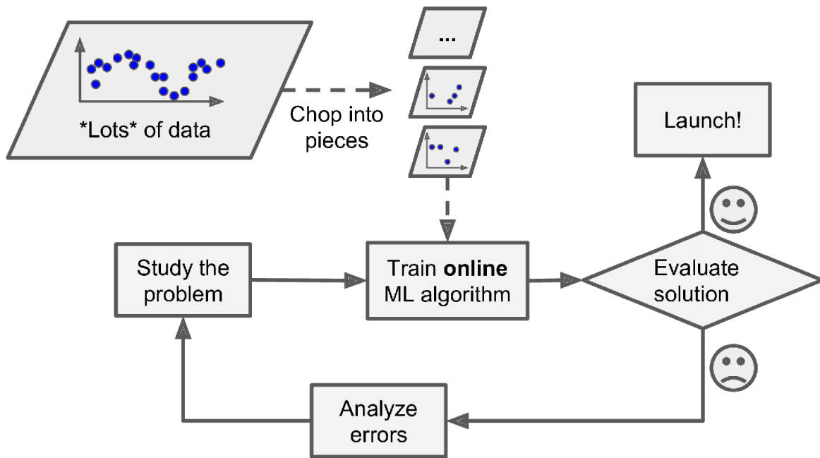
Figure 1-14. Using online learning to handle huge datasets
