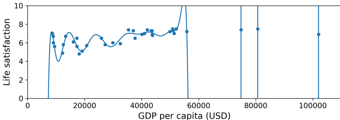
Figure 1-22. Overfitting the training data
