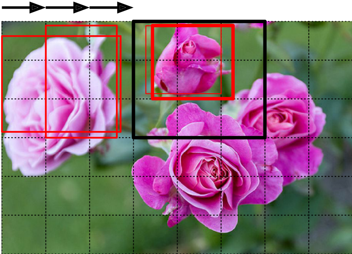
Figure 14-24. Detecting multiple objects by sliding a CNN across the image
