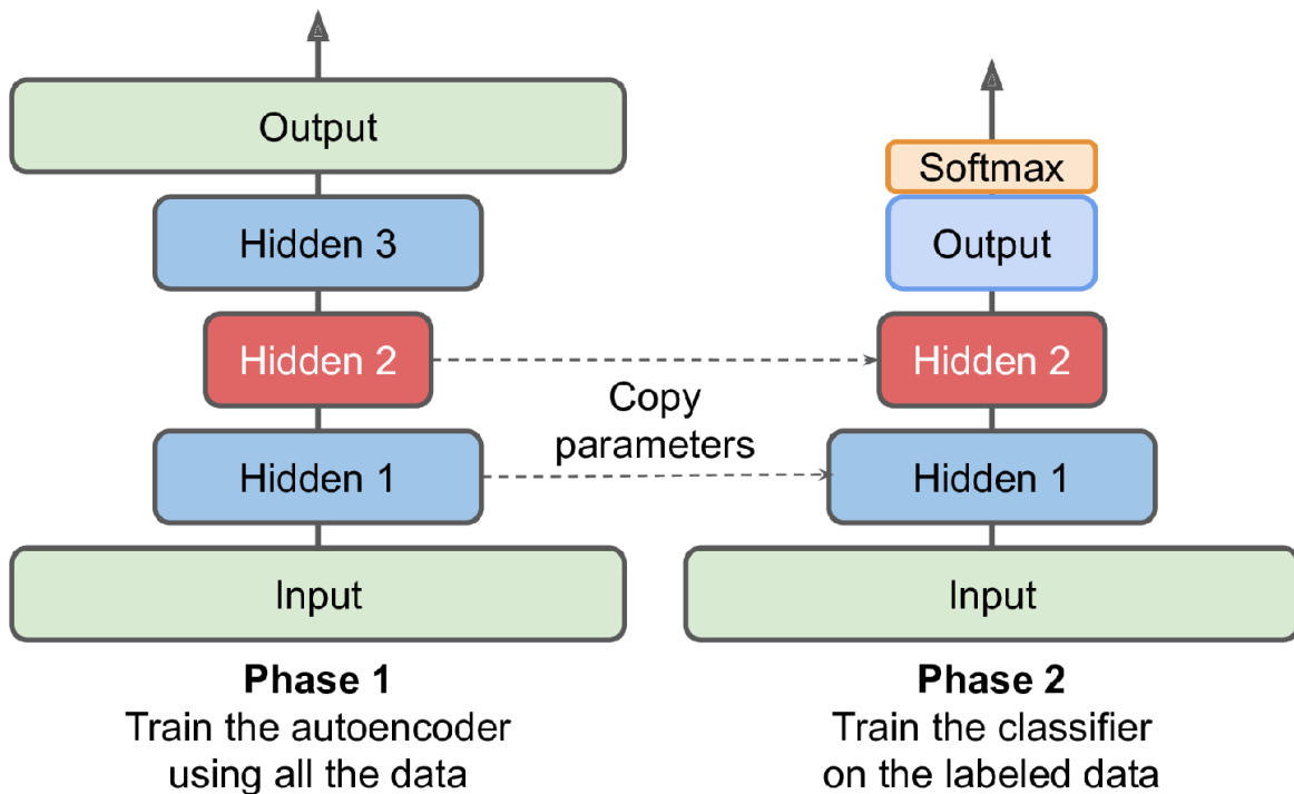
Figure 17-6. Unsupervised pretraining using autoencoders
