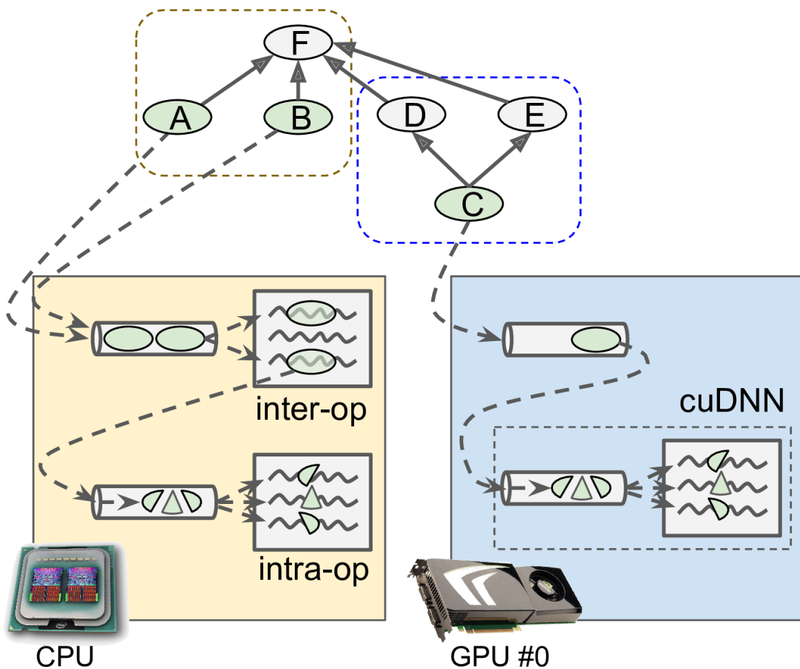
Figure 19-14. Parallelized execution of a TensorFlow graph
