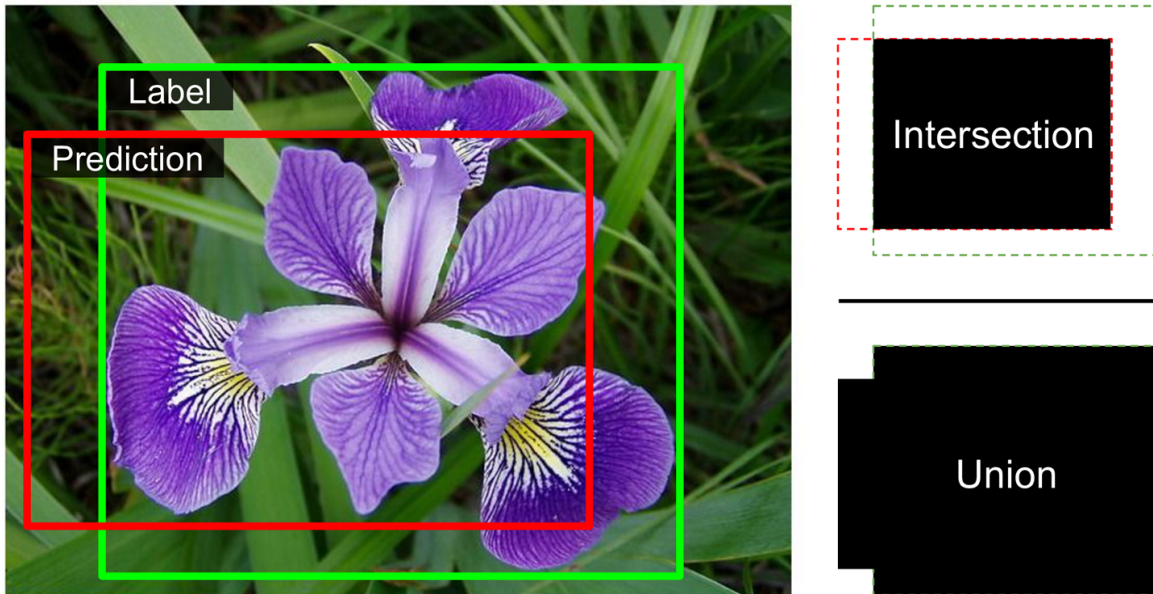
Figure 14-23. Intersection over Union (IoU) metric for bounding boxes
