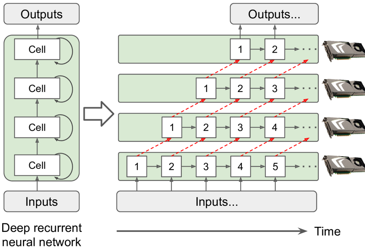
Figure 19-17. Splitting a deep recurrent neural network
