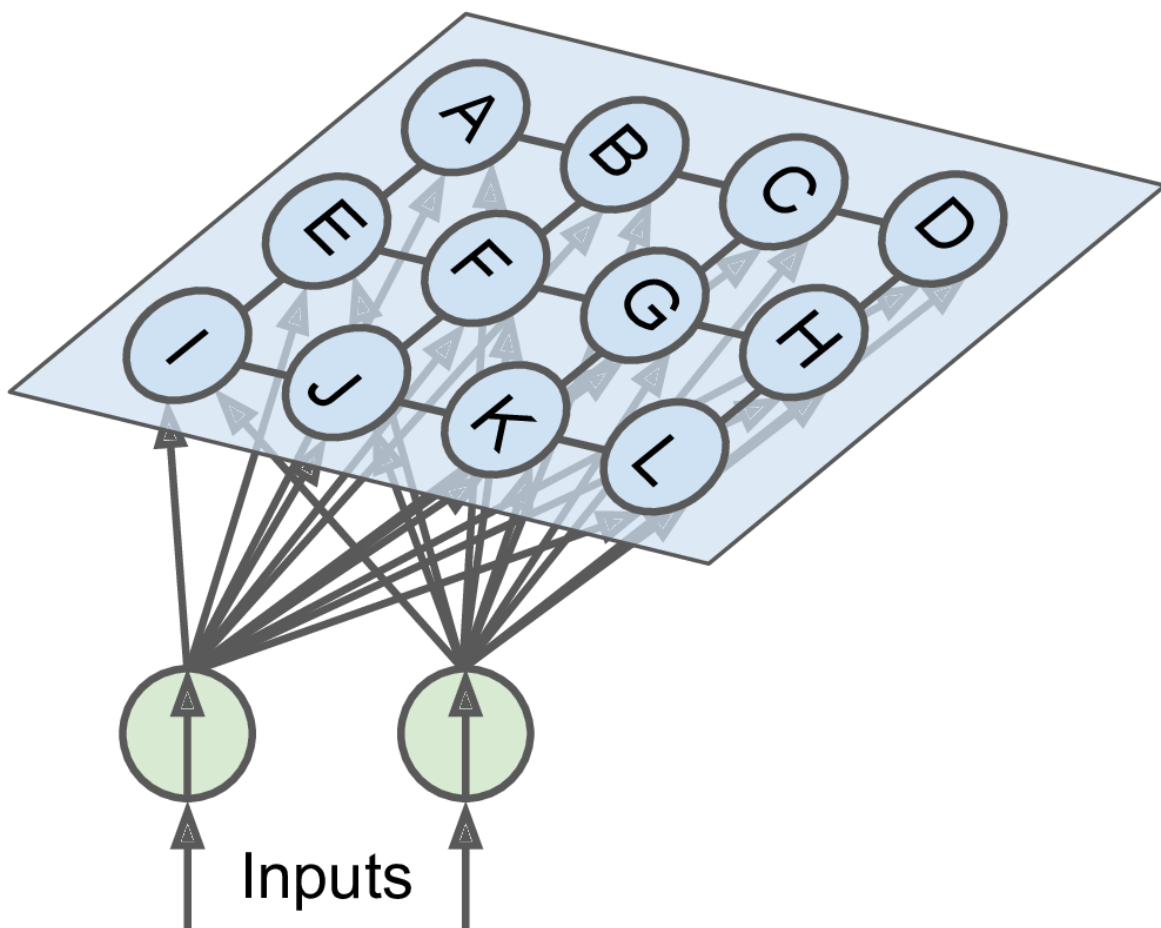
Figure E-5. Self-organizing map
