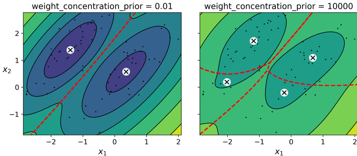
Figure 9-23. Using different concentration priors on the same data results in different numbers of clusters
