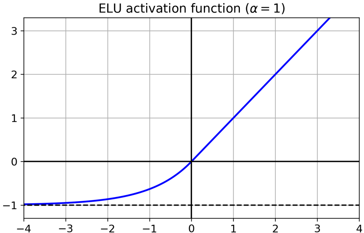
Figure 11-3. ELU activation function
