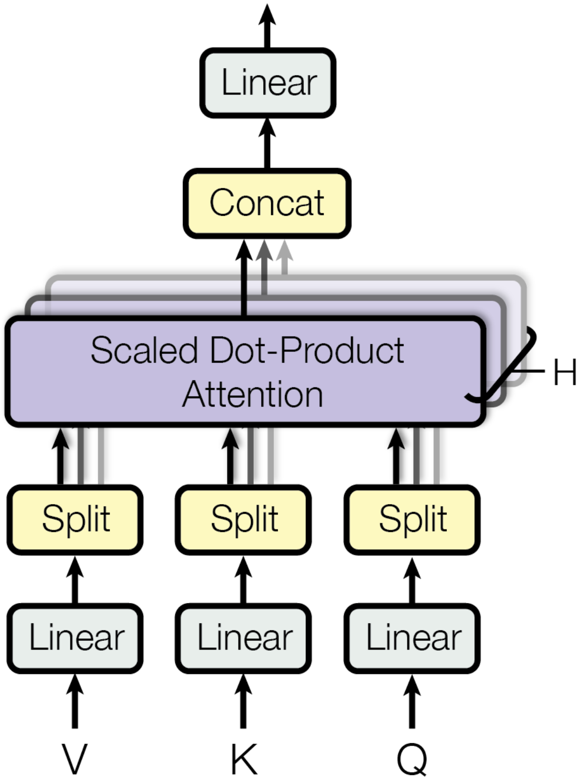
Figure 16-10. Multi-Head Attention layer architecture 23
