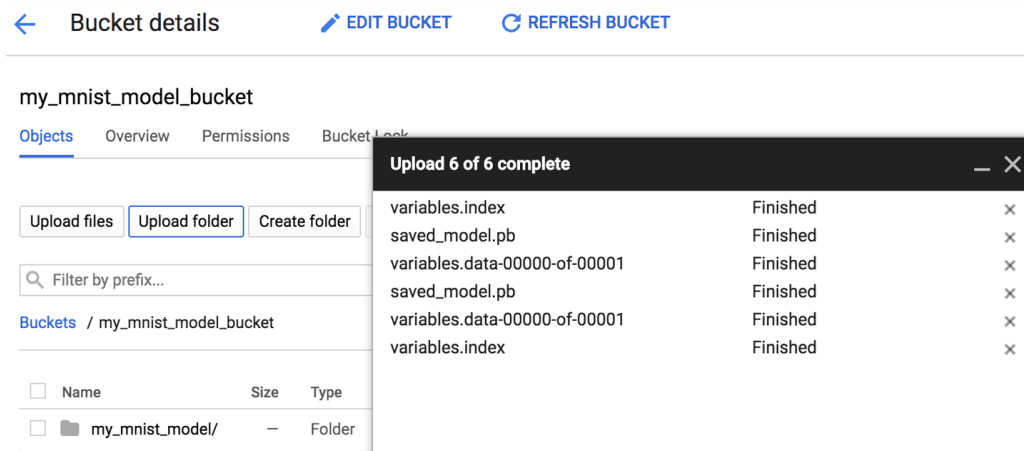
Figure 19-4. Uploading a SavedModel to Google Cloud Storage
