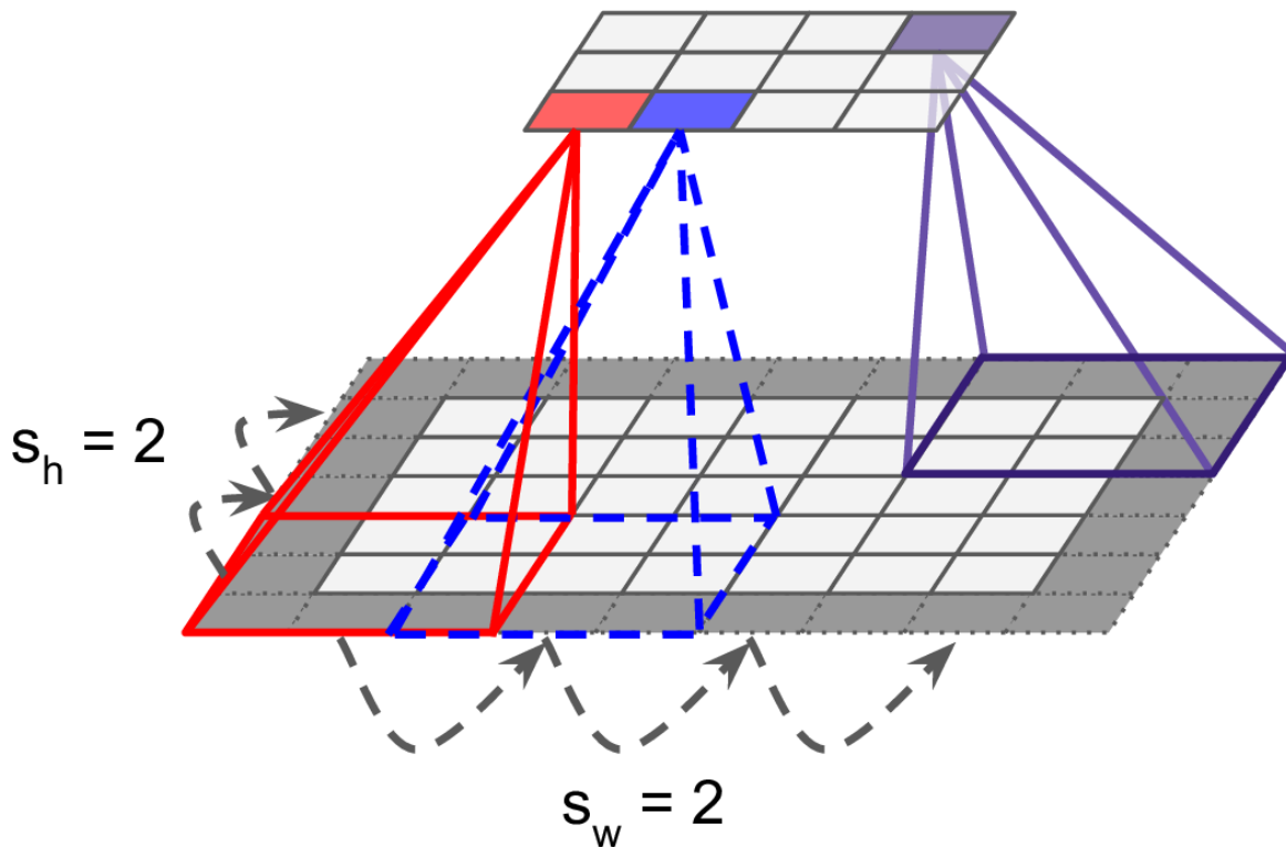
Figure 14-4. Reducing dimensionality using a stride of 2
