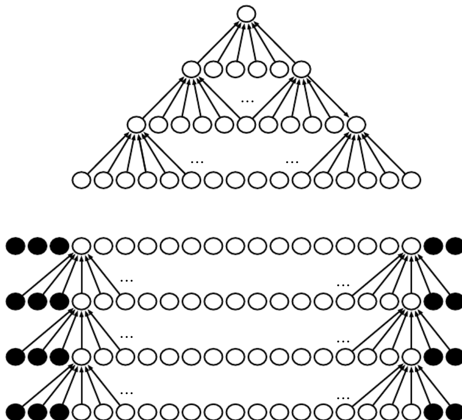
Figure 9.13: The effect of zero padding on network size : Consider a convolutional network with a kernel of width six at every layer. In this example, we do not use any pooling, so only the convolution operation itself shrinks the network size. ( Top ) In this convolutional network, we do not use any implicit zero padding. This causes the representation to shrink by five pixels at each layer. Starting from an input of sixteen pixels, we are only able to have three convolutional layers, and the last layer does not even move the kernel, so arguably only two of the layers are truly convolutional. The rate of shrinking can be mitigated by using smaller kernels, but smaller kernels are less expressive and some shrinking is inevitable in this kind of architecture. ( Bottom ) By adding five implicit zeroes to each layer, we prevent the representation from shrinking with depth. This allows us to make an arbitrarily deep convolutional network.
