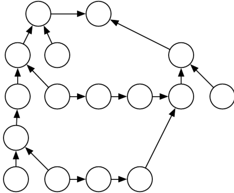
Figure 6.11: The computational graph used to compute the cost used to train our example of a single-layer MLP using the cross-entropy loss and weight decay.
