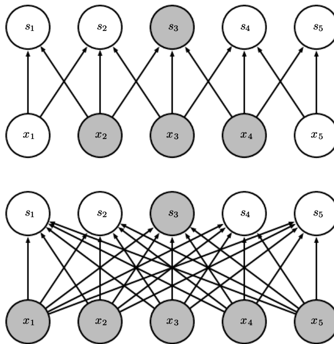
Figure 9.3: Sparse connectivity, viewed from above : We highlight one output unit, s_3 , and also highlight the input units in x that affect this unit. These units are known as the receptive field of s_3 . (Top) When s is formed by convolution with a kernel of width 3, only three inputs affect s_3 . (Bottom) When s is formed by matrix multiplication, connectivity is no longer sparse, so all of the inputs affect s_3 .
