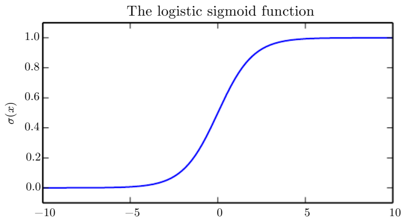
Figure 3.3: The logistic sigmoid function.
