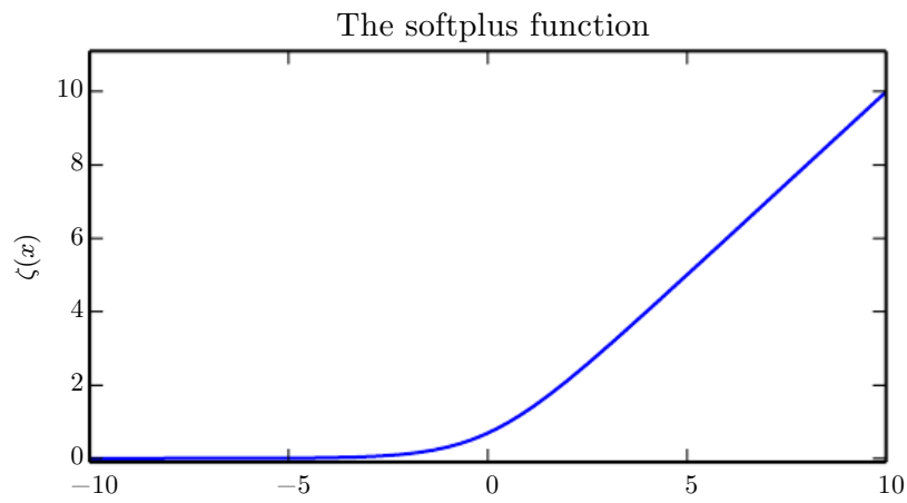
Figure 3.4: The softplus function.
