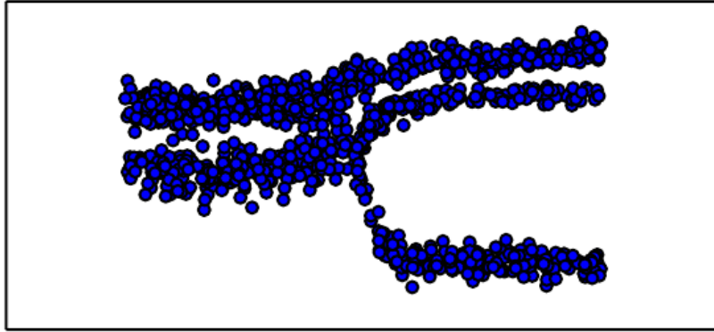
Figure 6.4: Samples drawn from a neural network with a mixture density output layer. The input x is sampled from a uniform distribution and the output y is sampled from p_{\text{model}}(y | x) . The neural network is able to learn nonlinear mappings from the input to the parameters of the output distribution. These parameters include the probabilities governing which of three mixture components will generate the output as well as the parameters for each mixture component. Each mixture component is Gaussian with predicted mean and variance. All of these aspects of the output distribution are able to vary with respect to the input x , and to do so in nonlinear ways.
